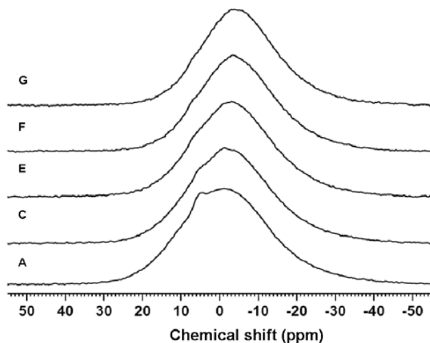
Figure 7: ^{23}\text{Na} MAS NMR spectra of glasses A, C and E to G.
