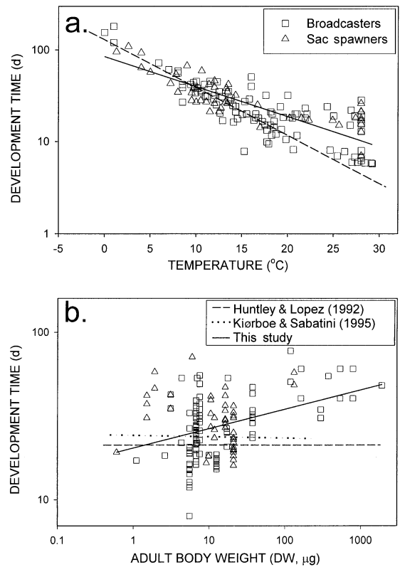
Fig. 3. (a) Development times for broadcast (□) and sac spawner (Δ) copepods as a function of temperature. Log regression of development time ( D , days) versus temperature (°C) from our results given by solid line, \log_e D = -0.076T + 4.438 ( r^2 = 0.666 , n = 151 , p < 0.001 ). (b) Development times for marine copepods as a function of adult body dry weight (DW, \mu\text{g ind.}^{-1} ), with development rates being corrected to 15°C using a Q_{10} value of 0.46 (as revealed by the analysis in Fig. 3a). For comparison, the laboratory ‘food saturated’ relationship of Kiørboe & Sabatini (1995) is given as a dotted line, and the ‘commonly food saturated’ relationship of Huntley & Lopez (1992) is given as a dashed line
