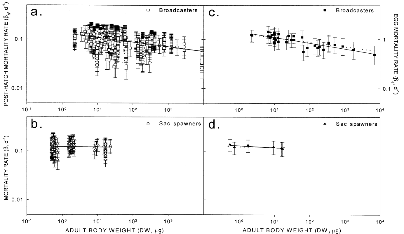
Fig. 5. Copepod mortality rate ( \beta , d^{-1} ) as a function of adult body dry weight (DW, \mu g ind. ^{-1} ). (a) Broadcast spawners ( \square ). The regression line is \log_{10}\beta = -0.092\log_{10}DW + 0.126 ( r^2 = 0.185 , n = 885 , p < 0.001 ) for eggs and \log_{10}\beta = -0.092\log_{10}DW - 0.874 for post-hatch individuals (solid line). (b) Sac spawners ( \triangle ). The regression line is \log_{10}\beta = -0.0085\log_{10}DW - 0.910 ( r^2 = 0.003 , n = 166 , p > 0.50 ns) (solid line). Vertical bars give the extent of the upper and lower prediction ranges (see text for details). Data corrected to 15°C using a Q_{10} -value of 2.0 (estimated from the analyses in Fig. 4). (c) Species means for broadcast spawners ( \blacksquare ). The regression line is \log_{10}\beta = -0.1174\log_{10}DW + 0.158 ( r^2 = 0.662 , n = 33 , p < 0.001 ) for eggs and \log_{10}\beta = -0.1174\log_{10}DW - 0.842 ( r^2 = 0.662 , n = 33 , p < 0.001 ) for post-hatch individuals (solid line). Dotted line gives regression from (a) for comparative purposes. (d) Species means for sac spawners ( \blacktriangle ). The regression line is \log_{10}\beta = -0.0387\log_{10}DW - 0.889 ( r^2 = 0.601 , n = 6 , p > 0.05 ns) (solid line). Dotted line gives regression from (b) for comparative purposes
