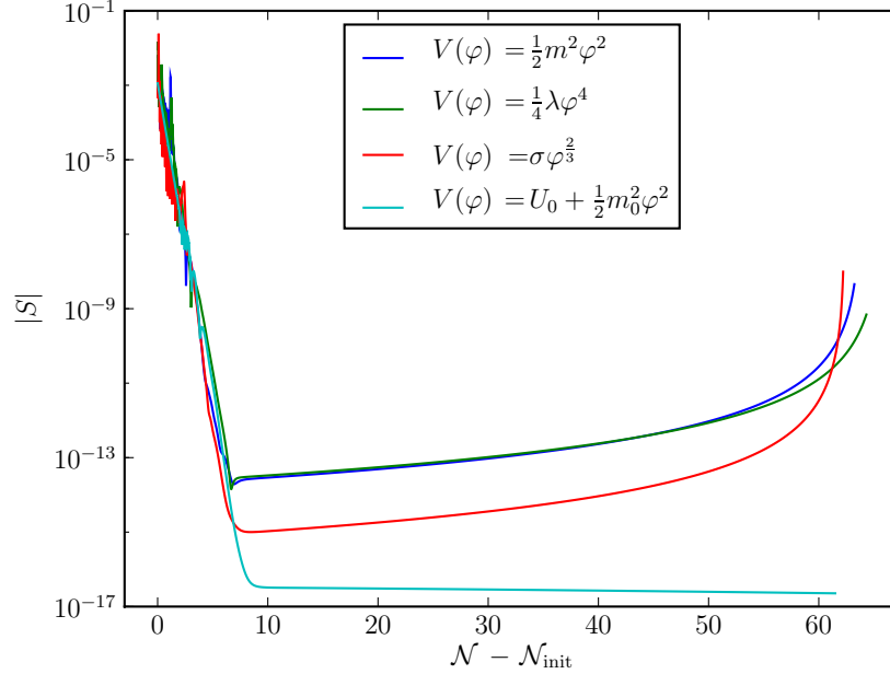
Figure 8.15.: Comparison of the source term evolution for the four different models. After horizon crossing the magnitude of the source term is larger for the quadratic and quartic models than for the other two. Towards the end of the numerical calculation there is a marked increase in |S| for three of the models as \bar{\epsilon}_H increases towards unity. The end time of inflation is specified by hand for the contrived toy model, so this effect is not seen.
