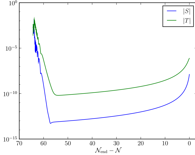
Figure 8.6.: The source term (lower blue line), as defined in Eq. (7.14), is compared with the T term (upper green line), as defined in Eq. (8.2), for k_{\text{WMAP}} . The source term is of comparable magnitude at the beginning of the simulation.
