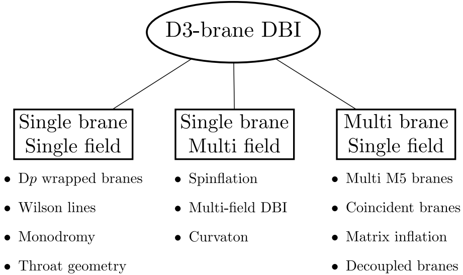
Figure 4.2.: A schematic of recent DBI inspired models
