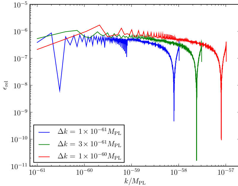
Figure 7.8.: The relative error in the integral I_{\mathcal{A}} for three different values of \Delta k . In contrast to Figure 7.7, k_{\text{min}} = 1 \times 10^{-61} M_{\text{PL}} = 3.8 \times 10^{-5} \text{Mpc}^{-1} \leq \Delta k for each case.
