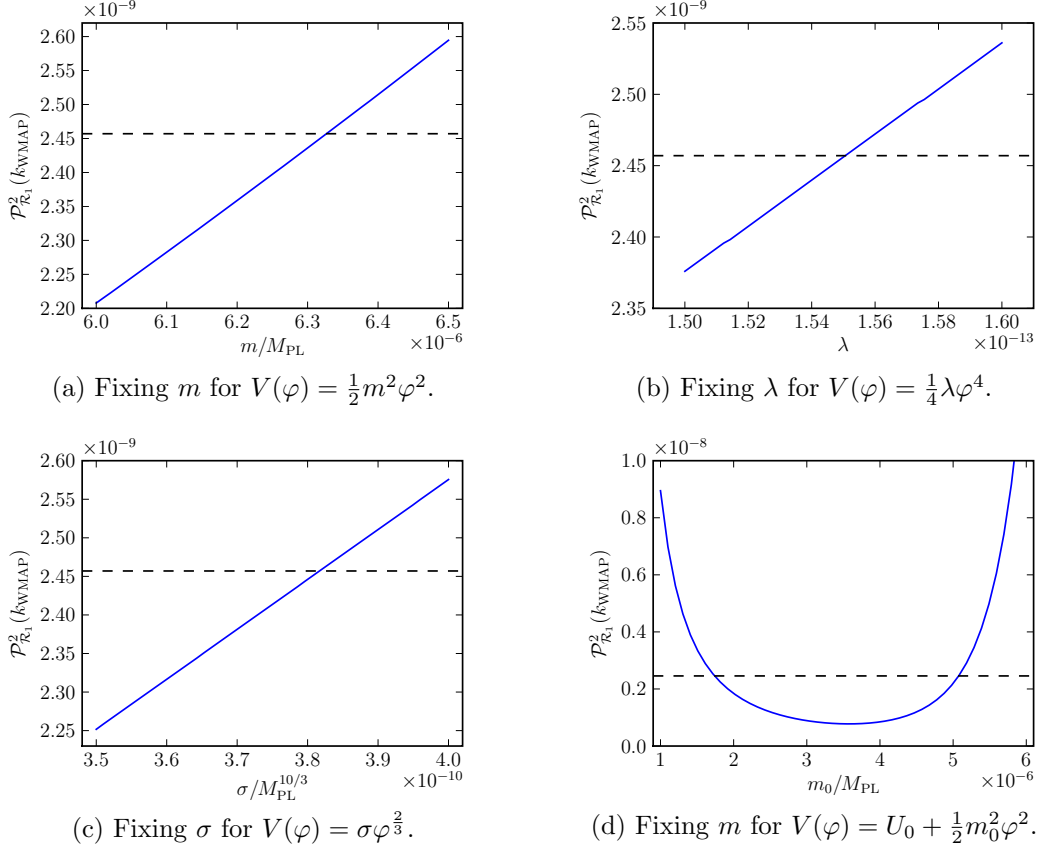
Figure 7.3.: Parameter values for the different potentials are chosen by requiring consistency with the WMAP5 normalisation of the first order power spectrum.
