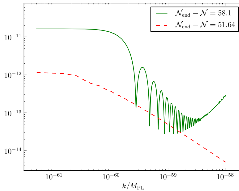
Figure 8.9.: The absolute magnitude of the source term for all k values in the range K_1 at two different time steps. The green line shows |S| when all modes have been initialised. The lower red dashed line shows |S| approximately 52 e-foldings before the end of inflation, when all modes have exited the horizon.
