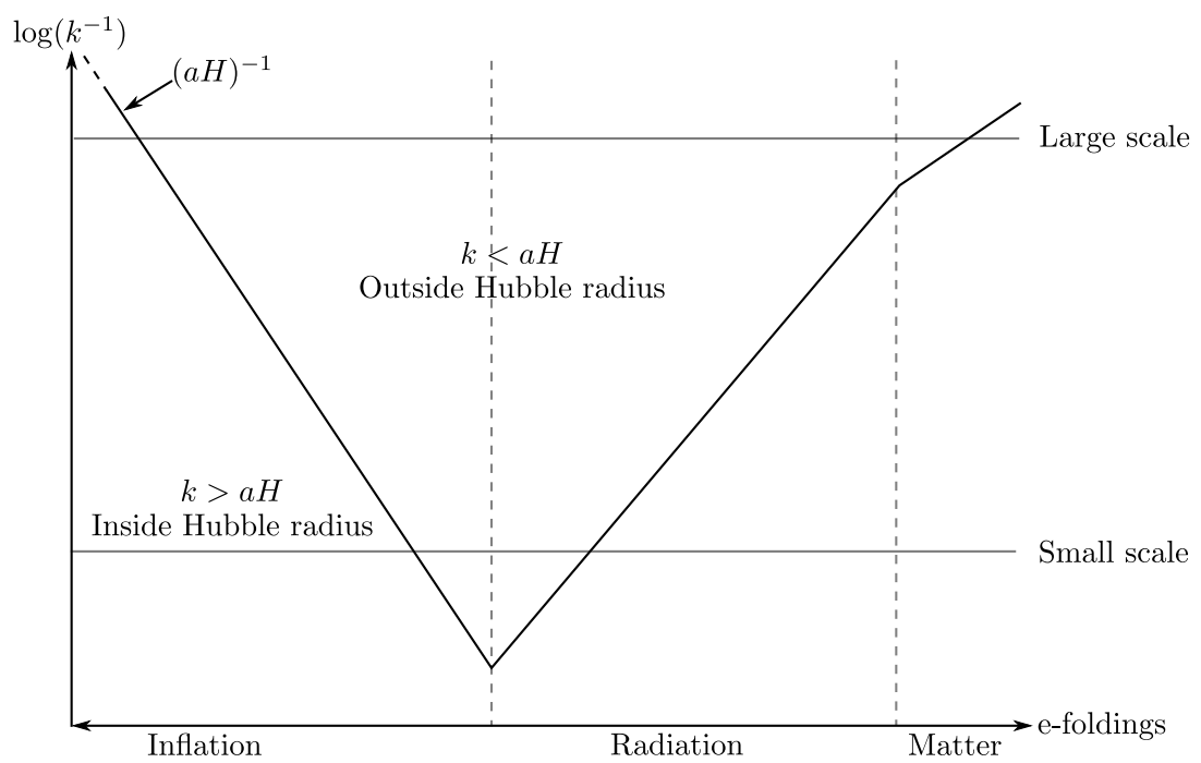
Figure 2.1.: Comoving scales that have recently entered the horizon would previously have been inside the horizon, if the inflationary period extended far enough into the past.
