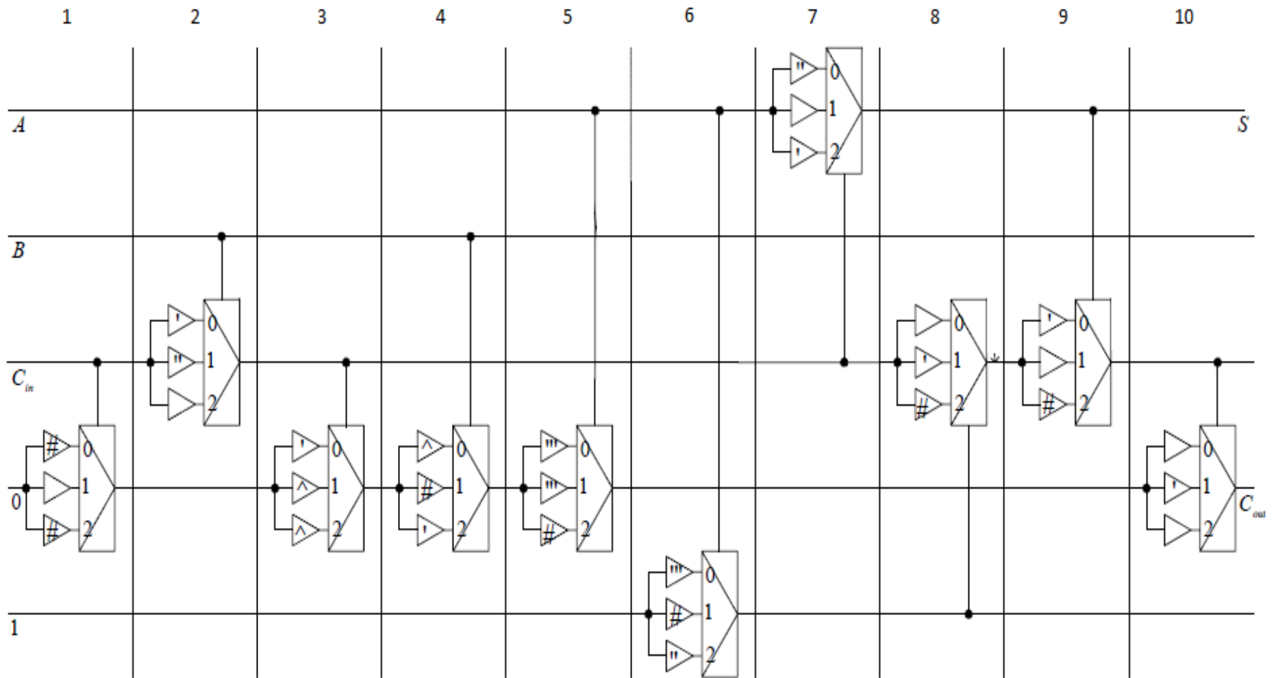
Figure: 19 Full Ternary adder
