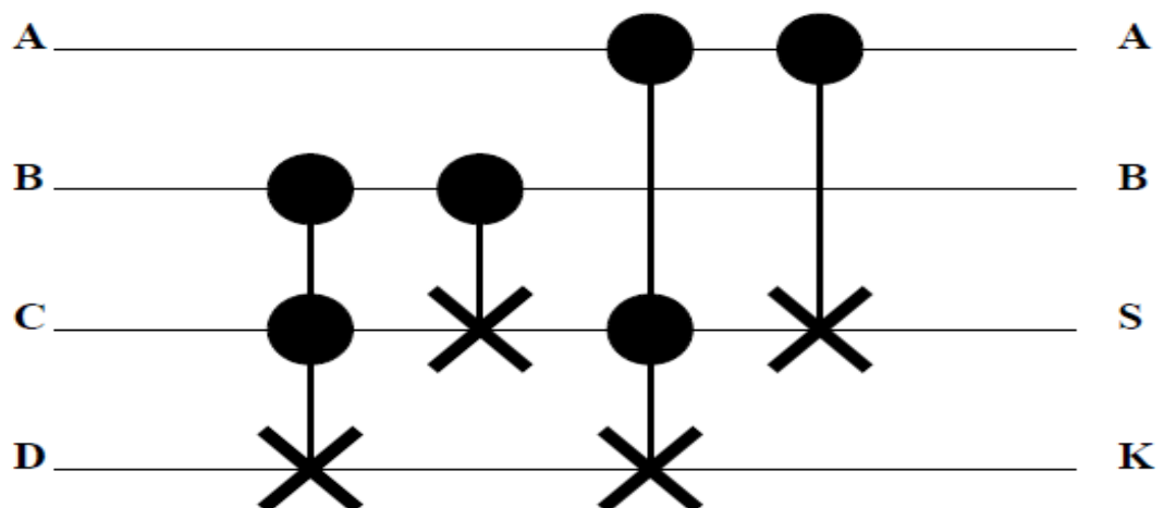
Figure 11: Quantum full adder
