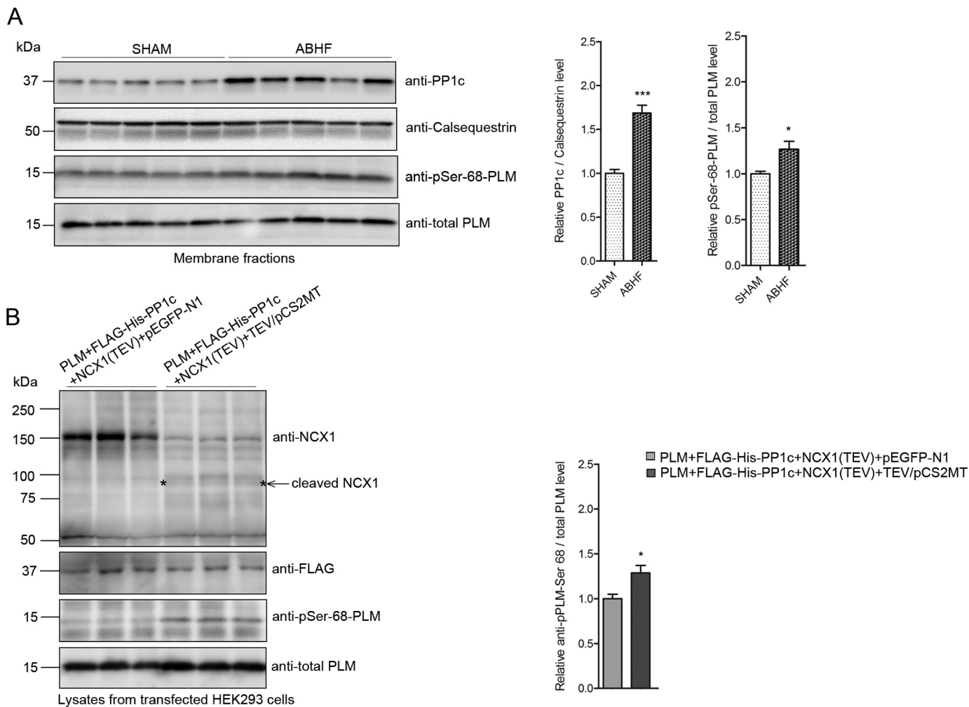
FIGURE 11. Analysis of NCX1, PP1c, and PLM in SHAM and ABHF rats. A , PP1c, pSer-68-PLM and PLM levels were analyzed in isolated cardiac membrane fractions by immunoblotting using relevant antibodies ( n = 5 ). Anti-calsequestrin and total PLM were used as loading controls. Bar graph show relative PP1c/calsequestrin level and pSer-68-PLM/total PLM level quantified by densitometry analysis. Differences were tested using unpaired t test (*, p < 0.05 ; ***, p < 0.001 ). B , FLAG-His 6 -PP1c(1–330), PLM, and NCX1 (TEV) were expressed with or without TEV protease followed by immunoblotting using relevant antibodies (in triplicates). Bar graph show relative pSer-68-PLM/total PLM level quantified by densitometry analysis. Differences were tested using unpaired t test (*, p < 0.05 ).
