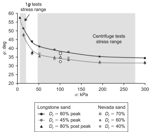
Fig. 8. Direct shear test results for Longstone sand: dependence of the angle of shearing resistance on stress level (Anastasopoulos et al. , 2010b). Friction angle for Nevada sand: evaluation from isotropically consolidated undrained compression tests at reference mean effective normal stress 100 kPa (Arulmoli et al. , 1992). The stress ranges at a depth equal to one foundation width are also depicted. The lower bound corresponds to the geostatic stress at this depth. The upper bound includes the geostatic stress and the stress induced by the structure dead weight
