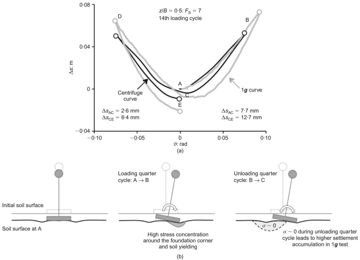
Fig. 16. (a) Settlement–rotation curve for the last loading cycle on the z/B = 0.5 profiles and comparison of settlement induced in each half cycle; (b) schematic illustration of the loading–unloading sequence in the 1g test (not drawn to scale)
