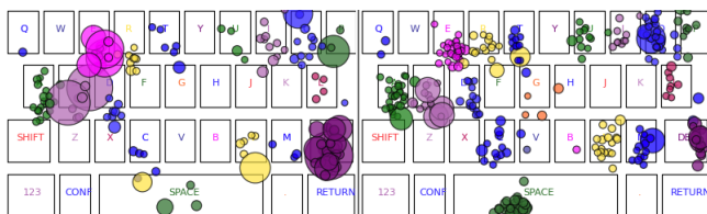
Figure 7. A Bubble indicates a pause; size represents its duration. Left - week 1 for P1, Right - week 8 for P1.
