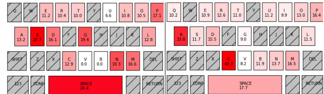
Figure 5. Substitution error rates per key. Gray keys were not used in the trials. Darker colors indicate higher error rates. Left - week 2, Right - week 8.
