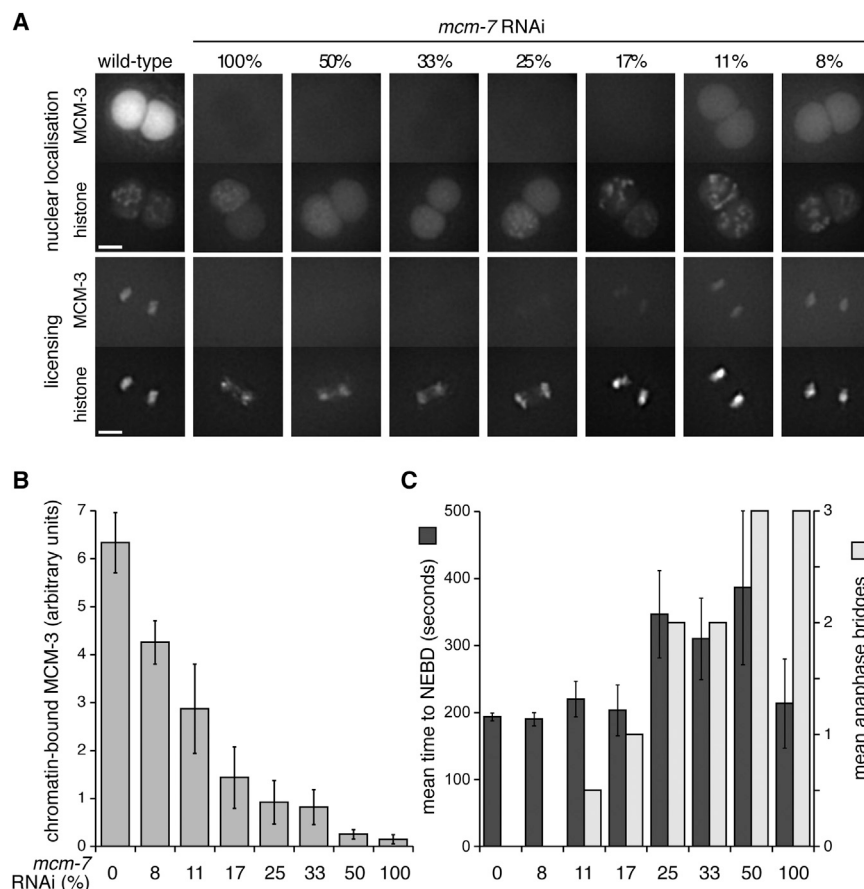
Figure 3. Graded Depletion of Chromatin Bound MCM-2-7
