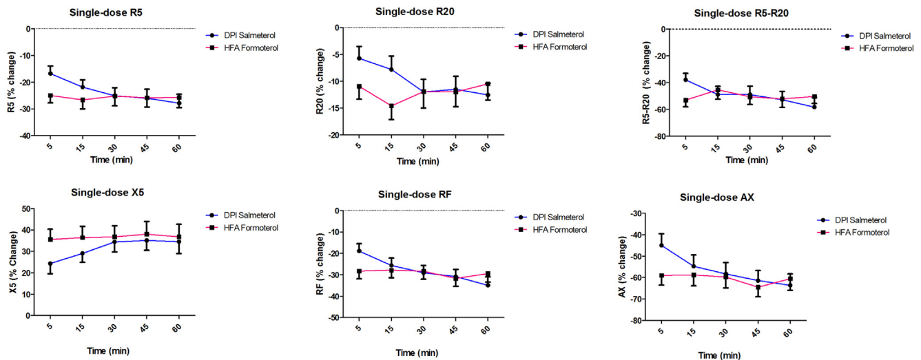
FIG 3. Effects on DPI IOS outcomes with either small-particle formoterol or large-particle salmeterol over a 60-minute period after inhaling the first dose shown as the percentage change from baseline. Data are depicted as means and SEMs. For all IOS outcomes, there were significant differences at 5 minutes, which were not sustained over the entire 60-minute period.
