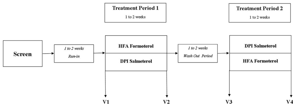
FIG 1. After a 1- to 2-week run-in period, patients received either 12 \mu\text{g} of small-particle HFA-formoterol or 50 \mu\text{g} of large-particle salmeterol dry powder 1 puff twice daily for 1 to 2 weeks each, with a 1- to 2-week washout period in between. Visits 1 and 3 were to assess the first dose, and visits 2 and 4 were to assess the last dose. At each visit, measurements were made at baseline and then over 60 minutes after inhalation. DPI , Dry powder inhaler.
