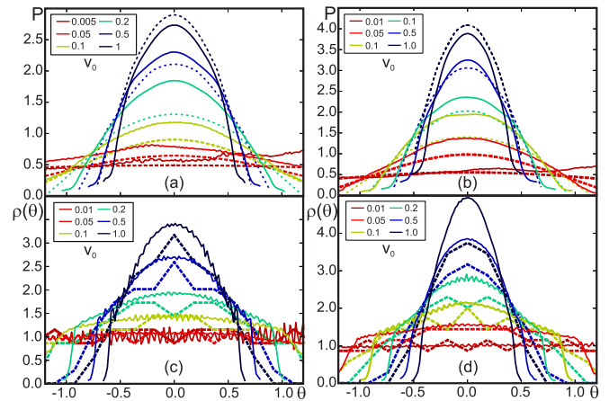
FIG. 7. (Color online) Simulation results (solid) and full chain calculation (dashed) compared to each other, for J = 1\tau^{-1} and s = 0.55 (a) and (c) and J = 0.1\tau^{-1} and s = 1.25 (b) and (d). Top row: pressure, and bottom row: density. Curves are ordered from flat to peaked with increasing v_0 , for both pressure and density, and also simulation and calculation results.
