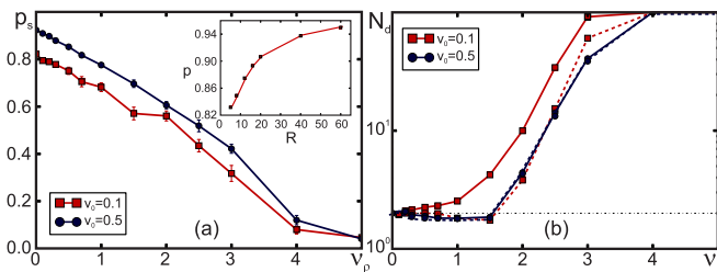
FIG. 12. (Color online) (a) Order parameter as a function of noise strength and velocity v_0 . The order linearly decreases with noise, but with no sign of a clear order-disorder transition. For the lowest v_0 , more complex band folding dynamics can be observed at low noise strengths, to be explored in detail elsewhere [44]. Inset: Order parameter as a function of radius. (b) Number of defects of the velocity field (solid) and the order parameter field (dashed) as a function of noise strength and velocity. From a value of 2 corresponding to the band state, first the velocity field and finally the order parameter field nucleate defect pairs until the band pattern abruptly disappears around v_r = 2.5\tau^{-1} .
