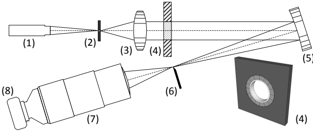
FIG. 1. Sketch of the optical setup: (1-3) laser and beam expansion system. A CPS196 adjustable focus ThorLabs 635nm diode laser (1) illuminates a \varnothing 15\mu\text{m} pinhole (2) located in the back focal plane of f_3 = 10\text{cm} lens (3); (4) the tunable acousto-optic hologram device; (5) R_5 = 50\text{cm} spherical mirror; (6) 0.3 mm edge; (7) AF-S NIKKOR 70-300mm zoom lens and ThorLabs KM100T CCD camera.
