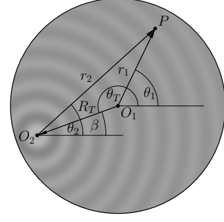
FIG. 2. Definition of coordinates systems used in Eq. (1).
