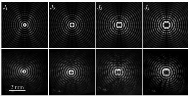
FIG. 3. intensity profiles of high-pass filtered Bessel beams of orders \alpha = 1 \dots 4 produced in simulation (top) and obtained experimentally (bottom).
