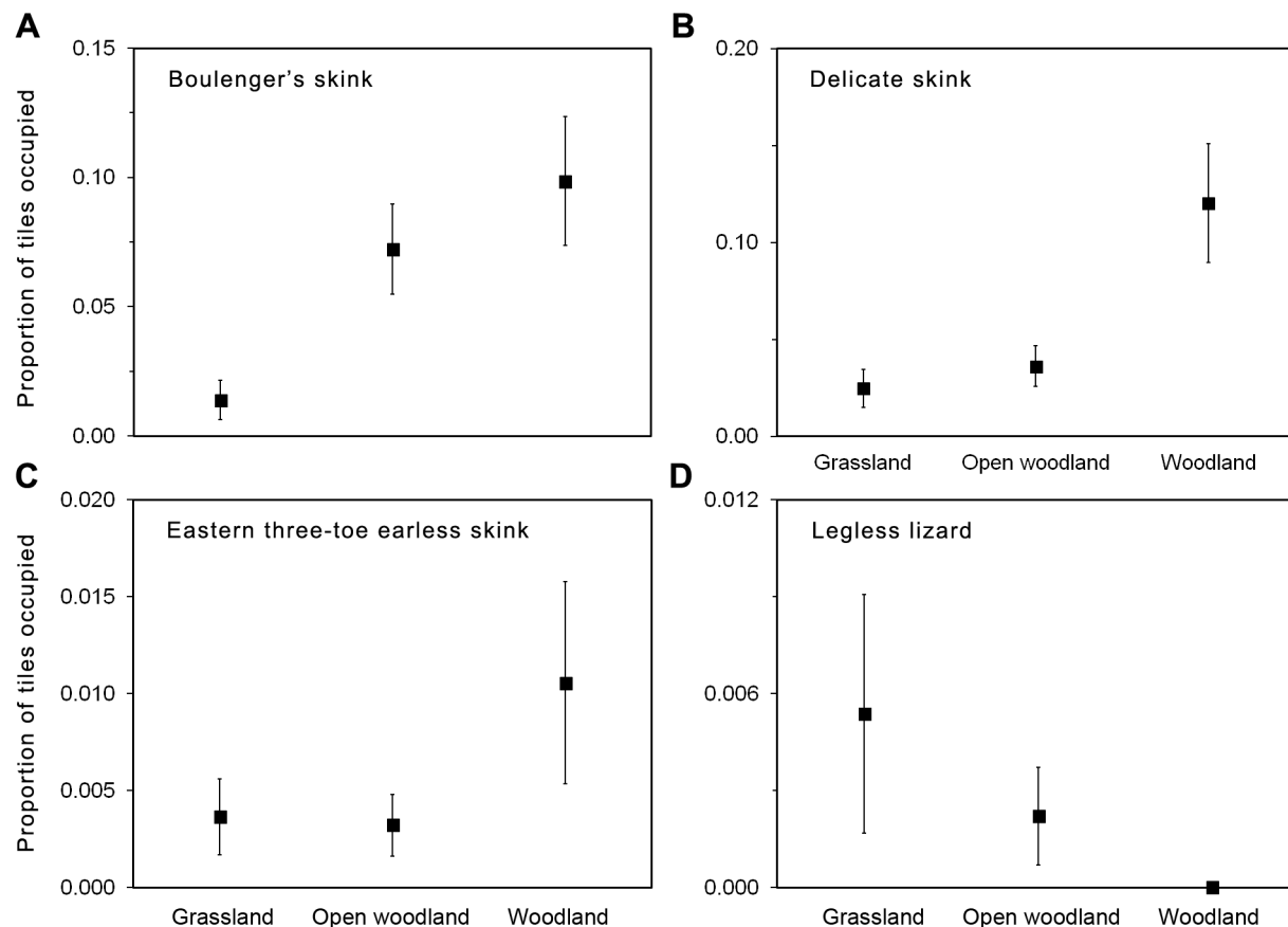
Figure 5. Graphical representation of logistic regression models summarized in Table 2. The graphs shows mean values for a) Boulenger's skink, b) delicate skink, c) eastern three-toe earless skink and d) legless lizard at a given plot for each tree canopy cover class (grassland, open woodland, woodland). Standard error bars are shown. To aid interpretation of results, variables have been back-transformed to original scale.
