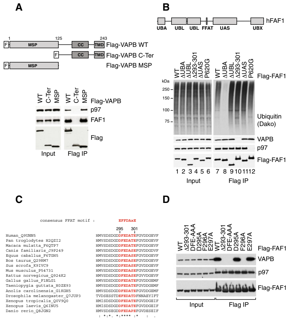
Figure 2 A FFAT-like motif mediates FAF1 interaction with VAPB. (A) The MSP domain of VAPB mediates its interaction with FAF1. Top panel: Schematic representation of the Flag-VAPB constructs, full length (1 to 243) or truncated, C-terminal half (125 to 243) and the MSP domain N-terminal half (1 to 125), immunoprecipitated from U2OS cells as shown in the bottom panel. Immunoblots of inputs (left) and immunoprecipitates (right) show that the MSP of VAPB is sufficient for the interaction with FAF1/p97. A highly conserved FFAT-like motif in FAF1 mediates its interaction with VAPB. (B) Top panel: Schematic representation of human FAF1 highlighting its various domains. Bottom panel: Wild-type or mutant variants of Flag-FAF1 were immunoprecipitated from U2OS cells. The indicated proteins were detected using specific antibodies in the inputs (left) and immunoprecipitates (right). UBA deletion caused a dramatic reduction in ubiquitinated protein binding to FAF1 whereas a point mutation in the UBX domain (P620G) abolished p97 binding. Deletion of the residues 293 to 301 was the only truncation that prevented VAPB binding to FAF1. (C) Alignment of FAF1 sequence from various species showing that the FFAT-like motif is highly conserved. (D) As in (B) , showing that either a triple mutation D295A/F296A/E297A or single F296A mutation in FAF1 abolished VAPB binding. IP, immunoprecipitate; WT, wild type.
