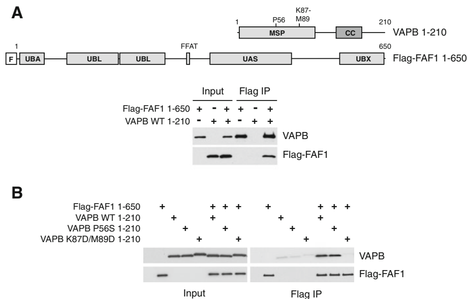
Figure 3 The P56S ALS-causing mutation of VAPB does not affect its interaction with FAF1 in vitro . The indicated variants of recombinant VAPB and Flag-FAF1 were incubated in vitro either alone or in combination, and then immunoprecipitated using anti-Flag beads. (A) Flag-FAF1 interacts directly with VAPB. Top panel: Schematic representation of the truncated version of VAPB (residues 1 to 210), lacking the C-terminal transmembrane region, and Flag-FAF1 full-length proteins expressed in bacteria. Bottom panel: Immunoblots of the indicated proteins in input extracts and anti-Flag immunoprecipitates. (B) The wild-type and the P56S mutant of VAPB (1 to 210), but not the K87D M89D double mutant, interact with Flag-FAF1 (right panel). IP, immunoprecipitate; WT, wild type.
