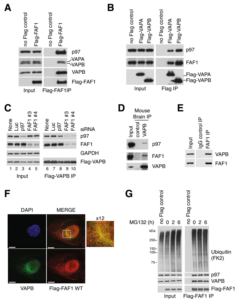
Figure 1 FAF1 interacts with VAPA and VAPB. (A) Flag-FAF1 immunoprecipitated from U2OS cells interacts with p97, VAPA and VAPB.
