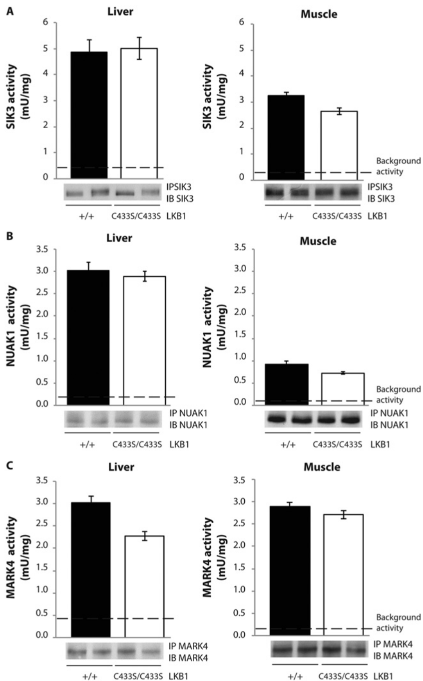
Figure S5 Activity of AMPK-related kinases in mouse tissues taken from wild-type LKB1 +/+ and LKB1 C433S/C433S mice
