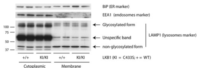
Figure S2 Liver cytoplasmic and membrane fractions from wild-type LKB1^{+/+} ( +/+ ) and LKB1^{C433S/C433S} (KI/KI) mice were immunoblotted with the indicated antibodies to determine the presence of endomembranes (endosomes, lysosomes and ER) in the cytoplasmic fraction preparation
