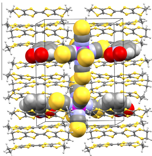
Fig. 2. View of the crystal packing of (\text{BEDT-TTF})_4[\text{Cr}(\text{NCS})_6]\cdot\text{C}_6\text{H}_5\text{NO}_2 viewed along the a axis with the b axis vertical, showing how the anions direct two isothiocyanate ligands towards the nitrobenzene molecules lying within the donor stacks.
