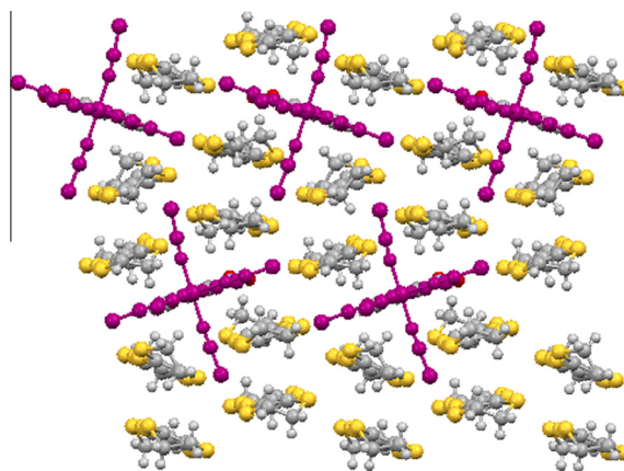
Fig. 3. View of the crystal packing of (\text{BEDT-TTF})_4[\text{Cr}(\text{NCS})_6]\cdot\text{C}_6\text{H}_5\text{NO}_2 viewed approximately along the c axis with the b axis vertical, showing the layer of [\text{Cr}(\text{NCS})_6]^{3-} anions lying over the BEDT-TTF/nitrobenzene layer. The nitrobenzene molecules lie directly behind the [\text{Cr}(\text{NCS})_6] anions.
