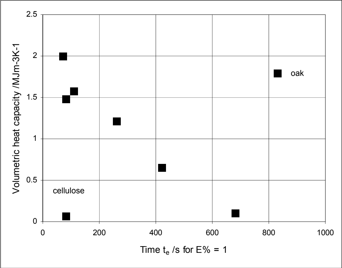
Figure 5: Graph of sample volumetric heat capacity against the E\% = 1\% times t_e .
