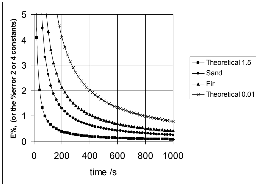
Figure 5: Graph of E\% , or the %error 2 or 4 constants plotted as a function of time for the theoretical materials with conductivities 1.5 and 0.01 W/mK, and for the sand and fir simulations. A 1% error or less is only possible after heating times of 70 s for Theoretical material 1.5, 260 s for sand, 420 s for fir and 780 s for the Theoretical 0.01.
