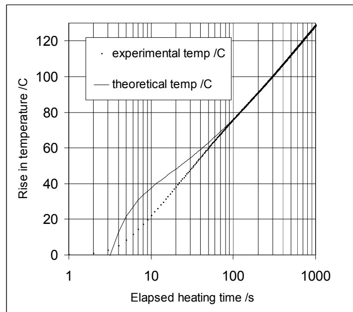
Figure 4: The Solver 4.2 predicted or theoretical temperature rise plotted with the Voltra simulation results, here denoted as experimental temp /C, both as functions of the elapsed heating time in seconds.
