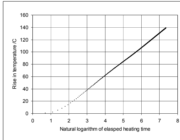
Figure 3: Graph of rise in probe temperature versus natural logarithm of elapsed heating time for the Voltra simulation on a theoretical material with conductivity 0.01 \text{ W/mK} , density 1000 \text{ kg/m}^3 , and specific heat capacity 100 \text{ J/kgK} . Temperature measured at 1\text{mm} from line heat source.
