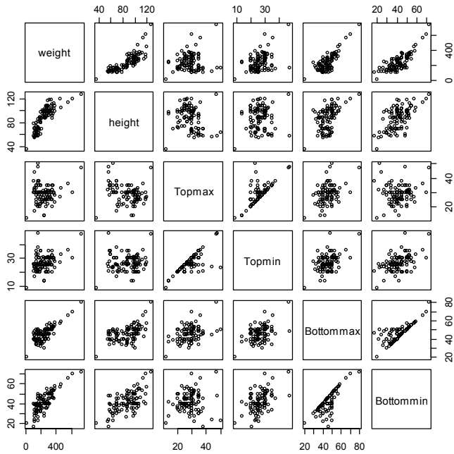
Fig. 4 – A “pairs” plot for six variables that characterise the loomweights, showing all possible bivariate plots. The upper triangle of plots is the same as the lower triangle, except that axes are interchanged. Treating the base and apex of the weights as rectangular, Topmax is the length of the larger sides of the rectangle at the apex and Topmin relates to the smaller side. Bottommax and Bottommin refer to similar dimensions for the base.
