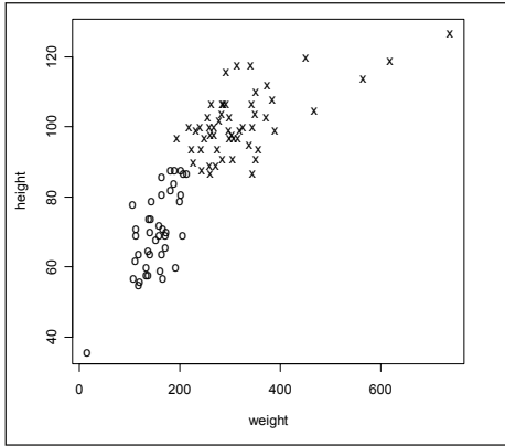
Fig. 12 – Similar to Fig. 6 but using all the data and with a modified size classification.
