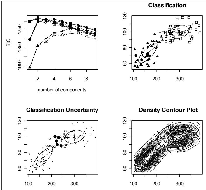
Fig. 9 – Assuming that the height/weight data can be modelled using a mixture of bivariate normal distributions, this figure shows different ways of displaying the results.
