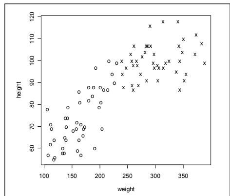
Fig. 6 – A plot of height against weight, with cases labelled by the classification suggested by the mixture analysis.
