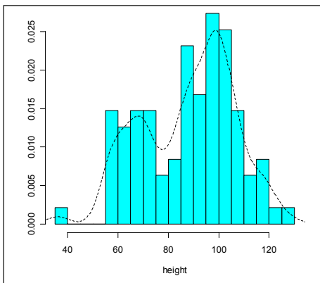
Fig. 5 – A histogram for the heights of the loomweights with a kernel density estimate superimposed.
