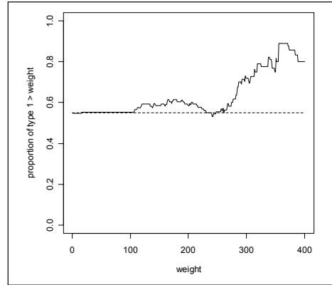
Fig. 13 – A graphic that suggests that Type 1 loomweights, with square tops and bottoms, are disproportionately likely to be of a heavier weight.
