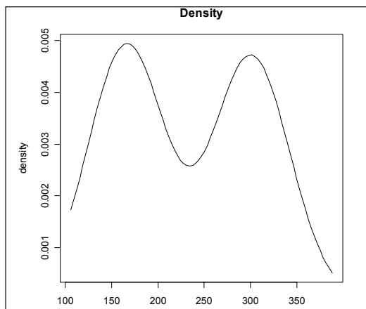
Fig. 3 – An estimated two-component normal mixture for the weights of the loomweights.
