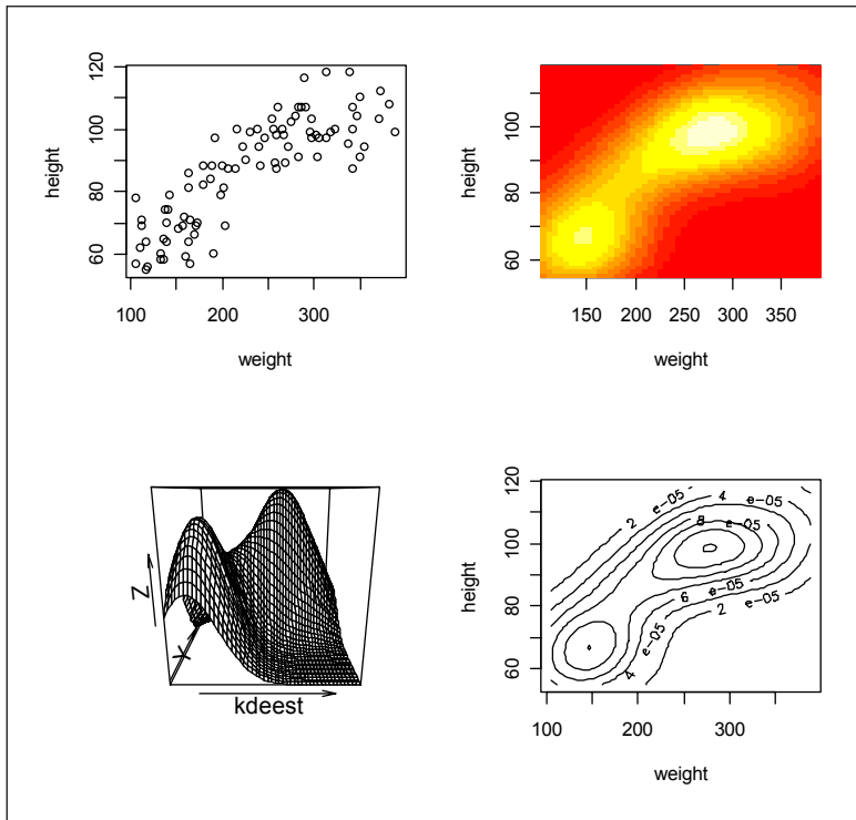
Fig. 7 – Different ways of displaying the relationship between height and weight. The raw data is to the upper-left; an image plot is to the upper-right; a perspective plot is to the lower left; a contour plot is to the lower-right.
