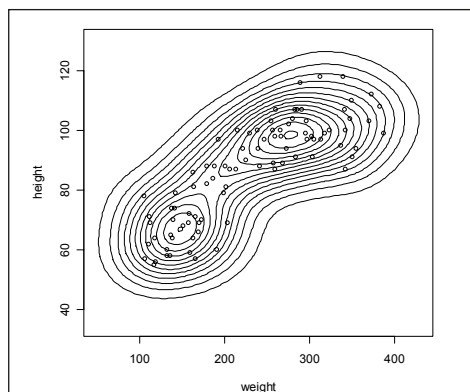
Fig. 8 – A customised version of the contour plot shown in Fig. 7.
