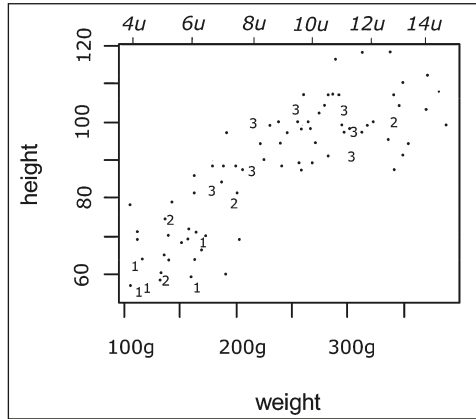
Fig. 15 – A plot of the modified dataset labelled with the Casa del Chirugo groups summarised in Tab. 1.
