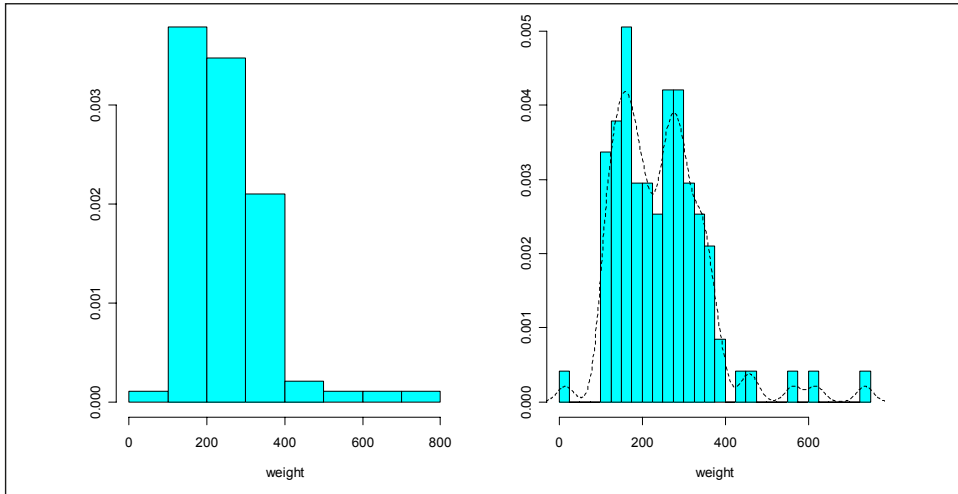
Fig. 2 – Two histograms using different bin-widths that show the distribution of weights of loomweights from Pompeii. That to the right suggests the distribution is bimodal.
