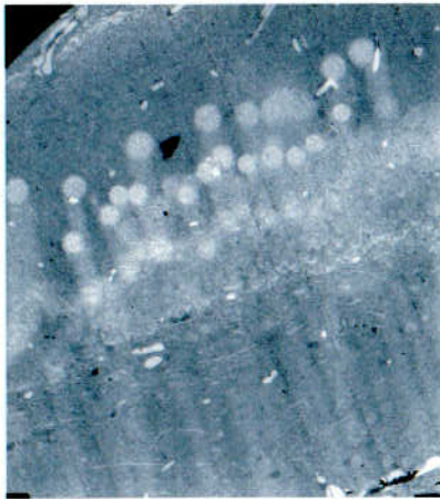
Figure 2.6 Volatilisation of resin by the electron beam of the Joel 1010 microscope.
