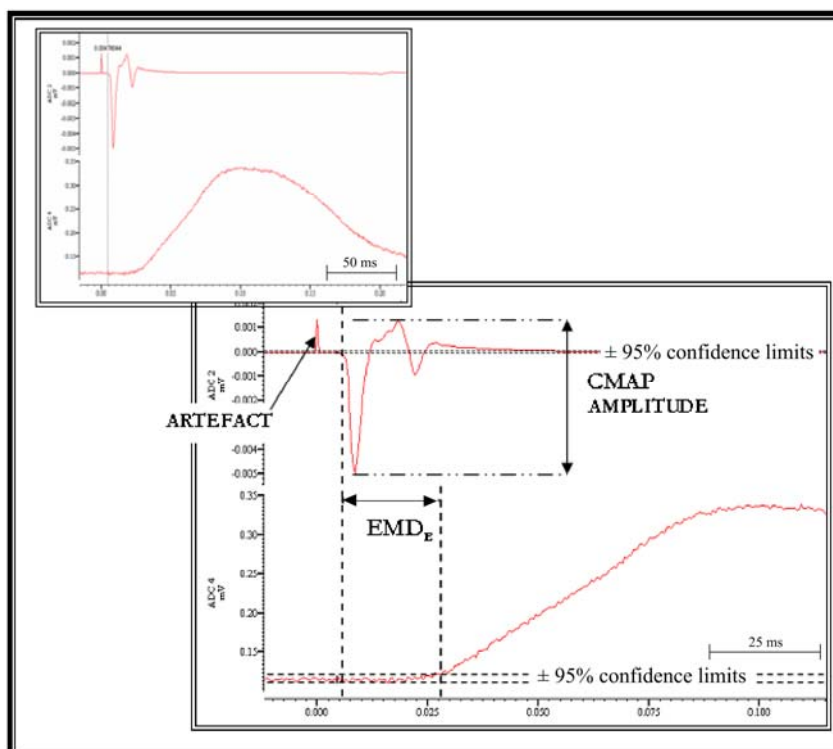
Figure 3. Example data showing; upper trace: example data of force and EMG associated with a single magnetic stimulus; lower trace: magnification of muscle activation to show representative calculation of magnetically-evoked electromechanical delay ( EMD_E ).
