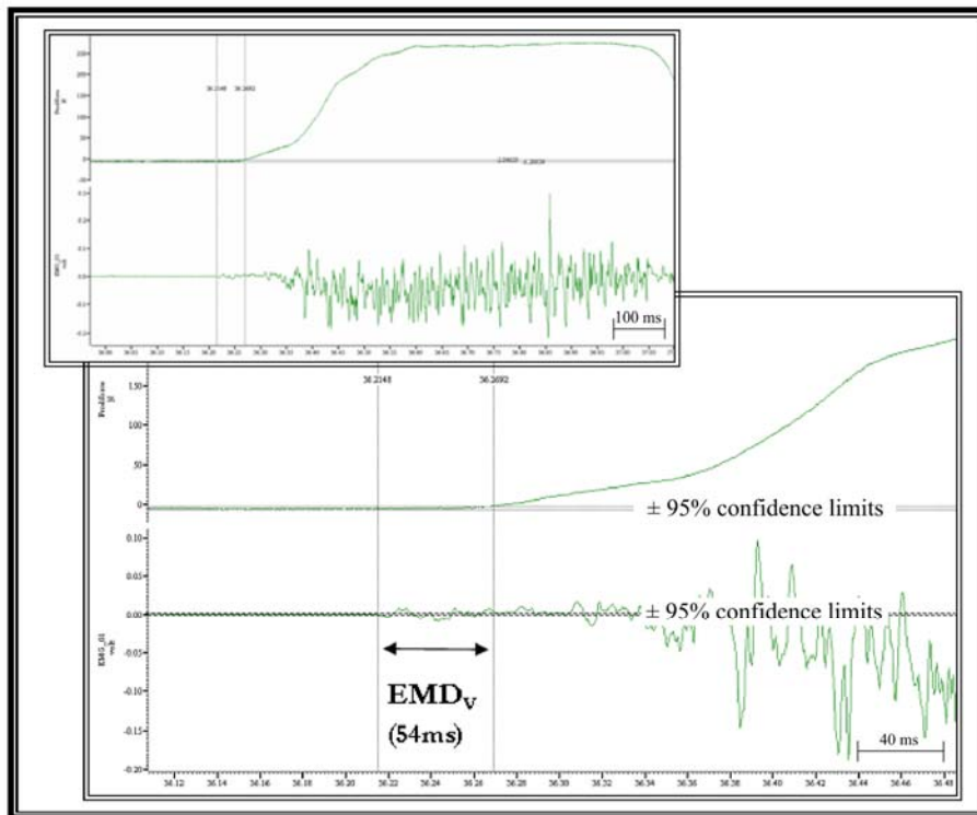
Figure 2. Example raw data showing: upper trace: example data of force and EMG associated with one MVMA; lower trace: magnification of muscle activation to show representative calculation of volitional electromechanical delay ( EMD_V ).
