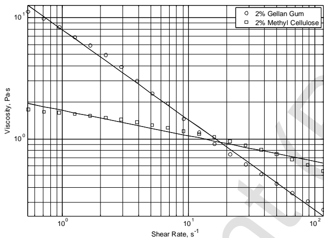
Figure 3: Log-log plot of viscosity against shear rate for gellan gum and methyl cellulose both at 2% w/v demonstrating near ideal behavior and allowing determination of consistency ( k_2 ) and power law index ( n ).
