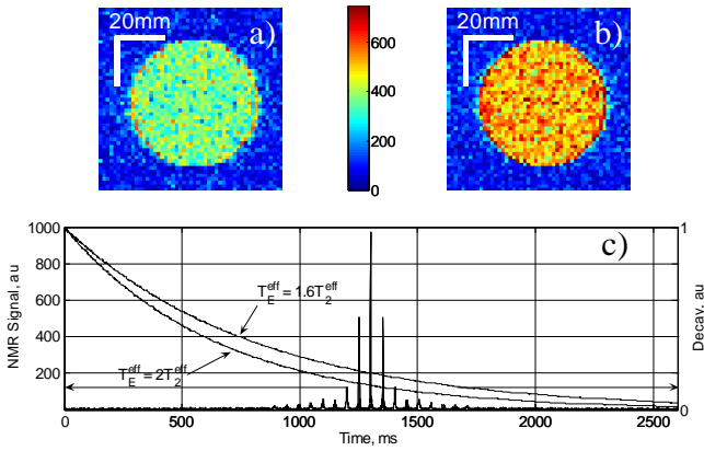
Figure 9: Demonstration of k-space clipping due to length of relaxation. a) image with T_E^{\text{eff}}=2T_2^{\text{eff}} ; b) image with T_E^{\text{eff}}=1.6T_2^{\text{eff}} ; The pixel intensities are in arbitrary units. c) shows the RARE echo train with no relaxation, superimposed with the relaxation curve for the case T_E^{\text{eff}}=2T_2^{\text{eff}} , and for the case T_E^{\text{eff}}=1.6T_2^{\text{eff}} (red curves).
