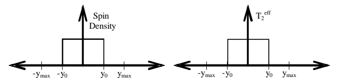
Figure 1: Simple homogeneous sample profiles used to estimate optimum echo time.
