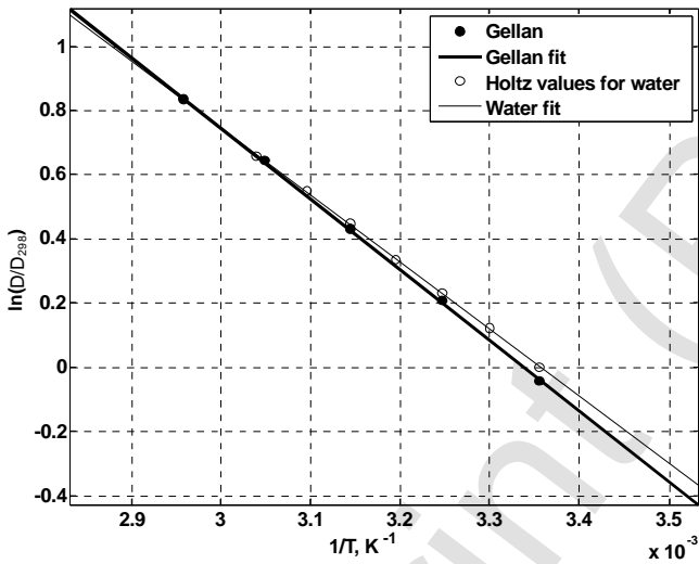
Figure 7: Plot of the natural logarithm of the diffusion coefficient against the reciprocal of temperature, normalized by value of bulk water at room temperature for water and gellan gum. Correlation between samples is high implying that the majority of water in the gel sample is unrestricted by the network.
