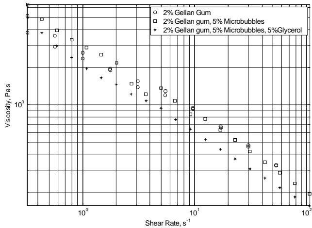
Figure 2: Log-log plot of viscosity against shear rate for the three samples. The addition of glycerol and microbubbles has little effect on the viscosity of the fluid, even at concentrations as high 5%. At low shear the viscosity of the fluids are very high with a value greater than 6Pa.s. The plot demonstrates near ideal power law behavior and allows determination of the rheological coefficients, consistency ( k_2 ) and power law index ( n ).
