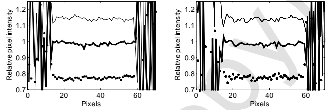
Figure 11: Horizontal (left) and vertical (right) profiles taken across the centre of MRI images in Figure 10. Broken line is for 0.95 bar, thick line for 1.3 bar and thin line for 1.44 bar.
