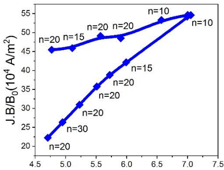
1 (a) \alpha (Normalized pressure gradient) (b) 2 Figure 4. Peeling-ballooning boundary of CFETR R=6.6\text{m} phase II in (a) J.B/B_0 versus \alpha_{ped} 3 space obtained from density scan in EPED , and (b) J.B/B_0 versus pedestal height space. The 4 density is scaled by 10^{19} \text{ m}^{-3} .
