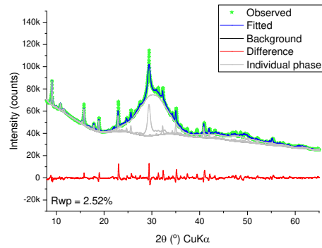
(b) 0% MgO
