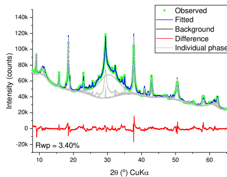
(e) 20% MgO
