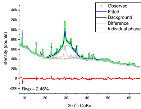
(c) 5% MgO
