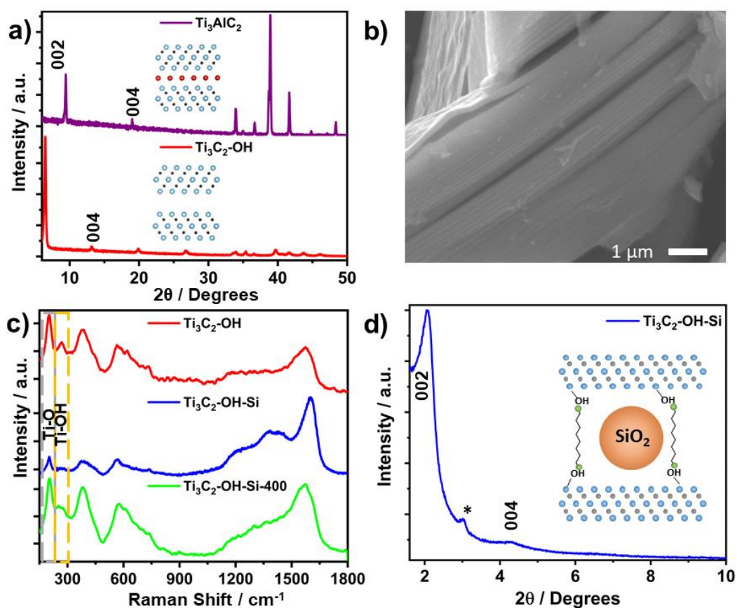
Figure 2. a) XRD patterns of the as made Ti 3 AlC 2 , Ti 3 C 2 after HCl washing (Ti 3 C 2 -OH). The (002) and (004) diffraction peaks were indexed according to Peng et al. 29 b) SEM micrograph of Ti 3 C 2 c) Raman spectra of the acid treated MXene (red, Ti 3 C 2 -OH), and the intercalated (blue, Ti 3 C 2 -OH-Si) and calcined at 400 °C (green, Ti 3 C 2 -OH-Si-400) pillared MXene, with dashed lines highlighting the key peaks corresponding to Ti-O (grey) and Ti-OH (orange) functional groups and d) Low angle XRD of the MXene after intercalation (Ti 3 C 2 -OH-Si). The asterisk highlights a peak corresponding to the glass sample holder (see SI Figure S9 for sample holder reference spectra).
