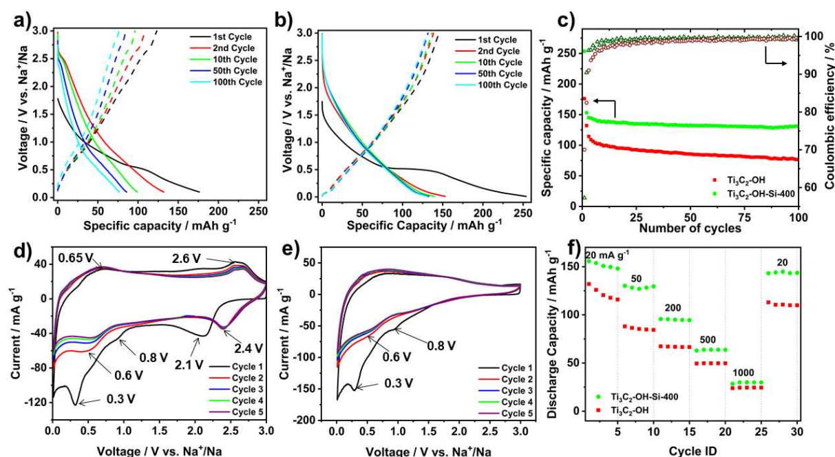
Figure 7. a-c) Galvanostatic data from half-cell tests against Na metal at 20 \text{ mA g}^{-1} in the voltage range 0.01-3 V. a) Load curves for selected cycles for a) \text{Ti}_3\text{C}_2\text{-OH} and b) \text{Ti}_3\text{C}_2\text{-OH-Si-400} , c) Coulombic efficiency and discharge capacities of the pillared and non-pillared samples over 100 cycles. d and e) Cyclic voltammograms at 0.01-3 V vs. Na metal at a scan rate of 0.2 \text{ mV s}^{-1} for d) the non-pillared, \text{Ti}_3\text{C}_2\text{-OH} and e) pillared MXene, \text{Ti}_3\text{C}_2\text{-OH-Si-400} . f) Rate capability tests for the pillared and non-pillared MXene at rates of 20, 50, 200, 500 and 1,000 \text{mA g}^{-1} . Five cycles are shown for each rate (one additional cycle at 20 \text{ mA g}^{-1} was conducted to ensure SEI formation).
