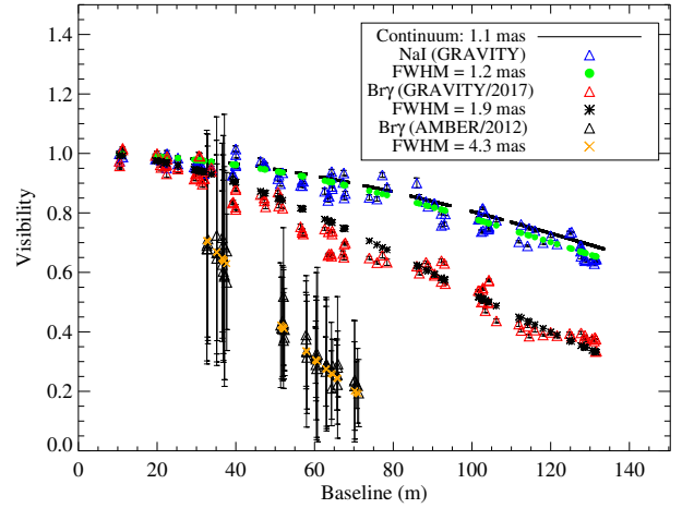
Fig. 12. Visibilities at the peak of the Bry, Na I emission lines and continuum emission towards IRAS 17163 overlotted with simple geometrical Gaussian models. Interestingly, Na I and continuum emission follow very similar distribution. Na I shows smaller drop in visibilities compared to Bry, indicating that Na I stems from a smaller emitting area compared to the Bry. The AMBER dataset was rebinned to match the spectral resolution of GRAVITY. A period of 5 yr indicates a shrinkage of the Bry emitting region to half size.
