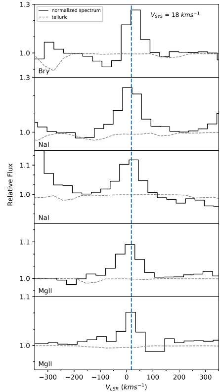
Fig. 4. Line profiles of the observed Bry, Na I and Mg II emission towards IRAS 17163. The dotted line represents the telluric absorption spectrum applied to correct the spectrum of the object. The vertical line represent the systemic velocity as reported by Wallström et al. (2015) using the optical Fe II emission.
