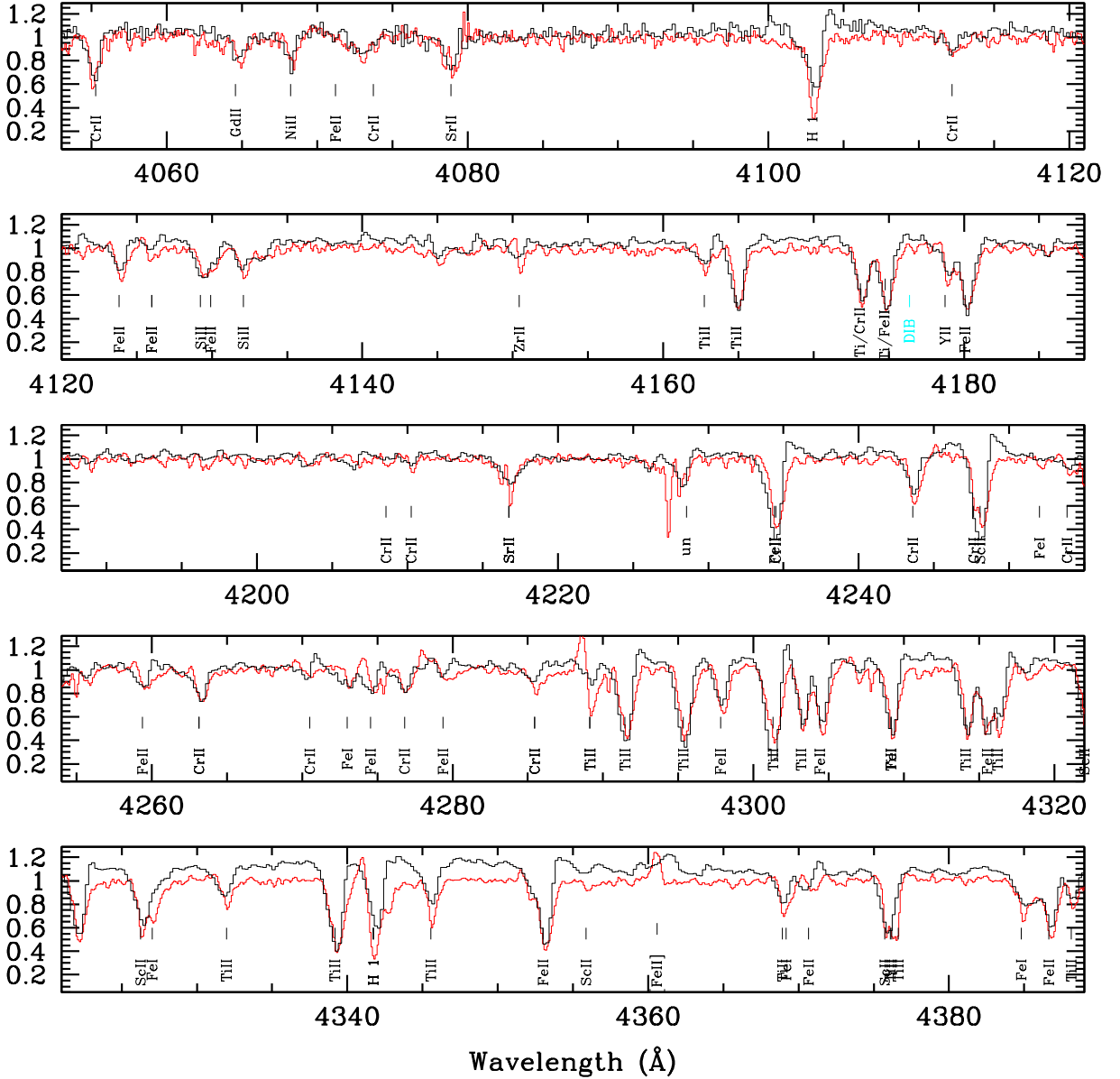
Fig. 10. Overlay of part of the blue spectrum of IRAS 17163 (black line) and IRC +10420 (red line). Note the tantalising similarity, as previously noticed also by Wallström et al. (2015) for the optical spectrum above 5000 Å which is dominated by emission lines.
