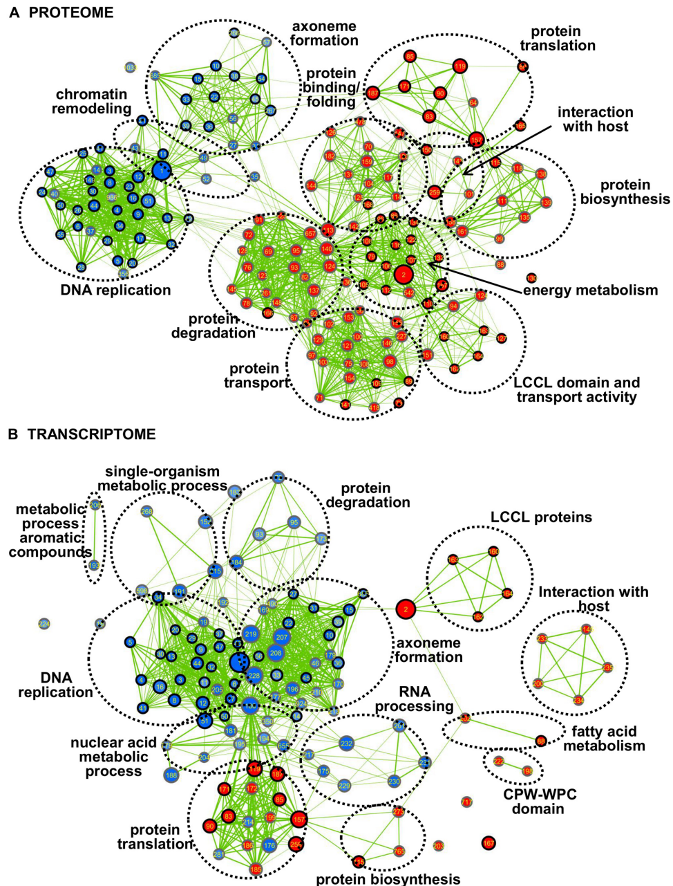
Figure 3. GSEA enrichment maps of protein and transcripts in purified P. falciparum MG and FG identifying gender-enriched biological networks. Enrichment maps from GSEA showing gene sets in an interaction network with nodes of (A) proteins or (B) transcripts in either MG (blue) or FG (red) with moderately conservative statistical significance ( p < 0.005 , FDR < 0.075 and overlap coefficient = 0.2). Clustered sub networks of nodes (depicted as dotted circles) reflect generic functional networks. Nodes represent enriched gene sets, where node size corresponds to the number of genes and colour intensity corresponds to statistical significance ( P -value). Edges represent overlap between gene sets with line thickness correlating to the degree of overlap. Gene sets identified in P. falciparum and P. berghei proteome are shown in (A) with node border colour in black. Gene sets identified in P. falciparum proteome and transcriptome are depicted in (B) with node border colour in black. Supplementary Table S7 provides the details of the GSEA analysis and the identification of the different nodes and edges.
