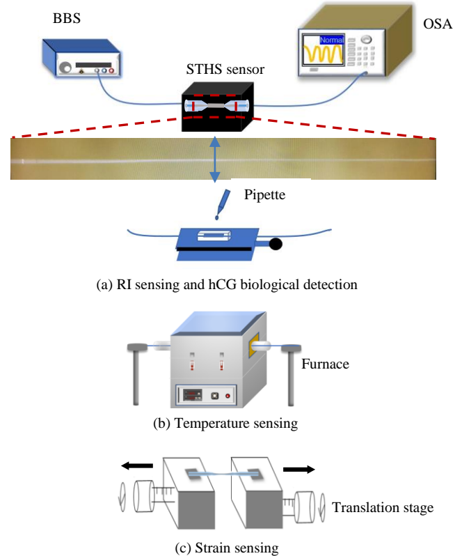
Fig. 3. The schematic diagram of the experimental setup (a) RI sensing and hCG detection, (b) temperature measurement and (c) strain sensing
