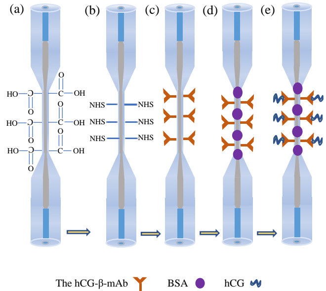
Fig. 6. Schematic diagram of fiber surface modification process: (a) treat with silane reagent to create carboxyl group; (b) generate NHS active ester with EDC/NHSS; (c) immobilize hCG-β-mAb on the fiber sensor surface; (d) block unbound sites with BSA; (e) specific binding with hCG.
