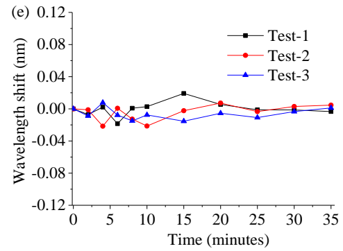
Fig. 4. Measured (a) spectral response of the sensor vs. RI variations at RI range of 1.33; wavelength shift of the sensor at RI range of (b) 1.33 (c) 1.37; (d) 1.41; and (e) stability tests of the sensor in PBS buffer.
