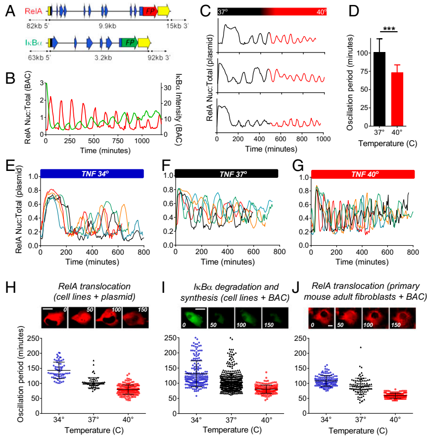
Fig. 1. Temperature sensitivity of the NF- \kappa B system. (A) Human BACs expressing RelA-DsRed xp and I \kappa B \alpha -EGFP. (B) Oscillations of RelA-DsRed xp and I \kappa B \alpha -EGFP degradation and resynthesis in a single human SK-N-AS cell (stably expressing both BACs) measured by confocal microscopy. (C and D) TNF \alpha -induced RelA-DsRed xp oscillation frequency increased significantly (** P < 0.01 ) following an increase in the incubation temperature (37 °C to 40 °C) surrounding the SK-N-AS cells (~8 h following TNF \alpha stimulation). Representative single-cell traces are shown (C). (E–G) Single-cell traces of TNF \alpha -induced oscillations in SK-N-AS cells transiently transfected with RelA-DsRed xp maintained at (E) 34 °C, (F) 37 °C, and (G) 40 °C. Cells were incubated at the respective temperature for 1 h before TNF \alpha stimulation. (H–J) Time-lapse confocal images and the distribution of the TNF \alpha -induced oscillatory period of NF- \kappa B in cells maintained at 34 °C, 37 °C, and 40 °C in (H) SK-N-AS stably transfected with RelA-DsRed xp (140 \pm 27 min; 100 \pm 17 min; 79 \pm 15 min, respectively), (I) SK-N-AS cells stably transfected with I \kappa B \alpha -eGFP BAC (132 \pm 42 min; 103 \pm 31 min; 79 \pm 12 min, respectively), and (J) mouse primary adult fibroblasts from transgenic mice expressing the RelA-DsRed xp BAC (108 \pm 17 min; 90 \pm 27 min; 59 \pm 9 min, respectively). P < 0.001 in all three cell models. Values show mean oscillation period \pm SD. (Scale bars, 10 \mu m.)
