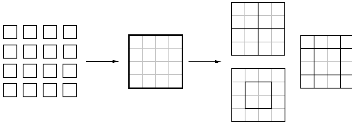
Figure 4. Squares array unification
