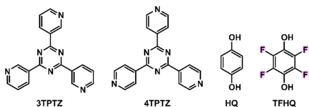
Fig. 1 Structures of the molecular building block used in this study: 2,4,6-tri(3-pyridyl)-s-triazine (3TPTZ), 2,4,6-tri(4-pyridyl)-s-triazine (4TPTZ), hydroquinone (HQ) and tetrafluorohydroquinone (TFHQ).
