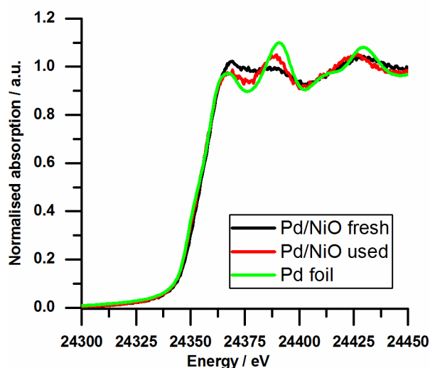
13 14 15 16 17 18 19 20 21 22 23 24 25 26 27 28 29 30 31 32 33 34 35 36 37 38 39 40 41 42 43 44 45 46 47 48 49 50 51 52 53 54 55 56 57 58 59 60 Figure 7. Pd K edge XANES of 1% Pd/NiO before and after reaction and a reference Pd foil.
