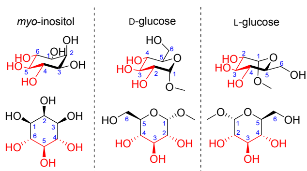
36 37 38 39 40 41 42 43 44 45 46 47 48 49 50 51 52 53 54 55 56 57 58 59 60 Figure 2: Structures of methyl \alpha -D-glucopyranoside and methyl \alpha -L-glucopyranoside relative to myo -inositol with the shared stereochemistry of the hydroxyl groups highlighted in red.
