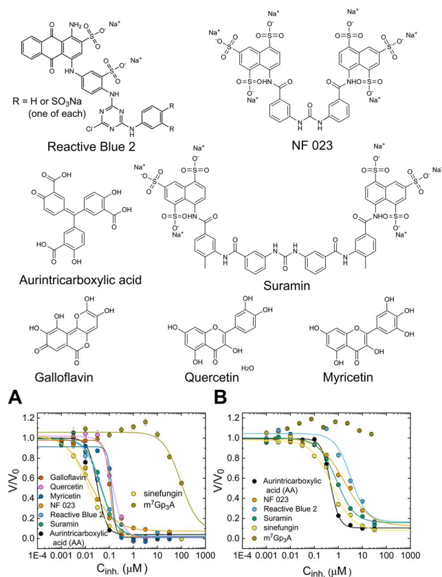
Figure 7. Inhibition of N7-MTase activities of A) Ecm1 and B) RNMT-RAM toward 6b by the most potent selected substrate analogs and sinefungin. All reaction mixtures contained probe 6b (2 \mu\text{M} ) and either SAM (50 \mu\text{M} ), Ecm1 (10 nM) or SAM (20 \mu\text{M} ), RNMT-RAM (20 nM) in 50 mM Tris-HCl buffer pH 7.5. The mixtures were incubated at 30 ^{\circ}\text{C} in a 96-well plate reader. The fluorescence measurements were carried out for excitation at 345 nm and emission at 378 nm. Data are the means \pm SD of two or three independent experiments. The determined \text{IC}_{50} and Hill slope values are shown in Table 4.
