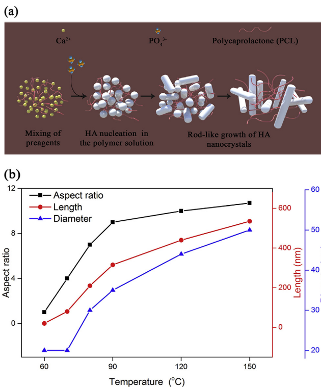
Fig. 7. (a) Schematic presentation of nucleation and growth of HA particles in the polymer matrix (PCL) during solvothermal processing in an alkaline solution (pH = 10). (b) Effect of temperature on the dimensions of in-situ synthesized HA particles.
