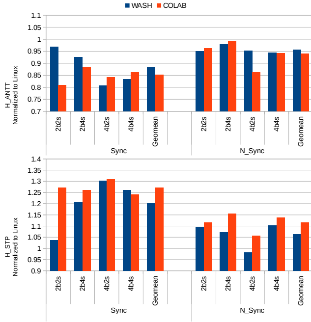
Figure 5. Performance of Synchronization-Intensive and Non-Synchronization-Intensive Workloads. All results are normalized to the Linux CFS ones. Lower is better for H_{ANTI} and higher is better for H_{STP} .
