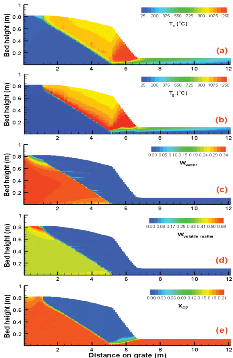
Figure 4. Main results from the model: (a) temperature of solid, (b) temperature of gas, (c) mass fraction of moisture in the solid, (d) mass fraction of volatile matter in the solid, and (e) mole fraction of oxygen in the gas phase.
