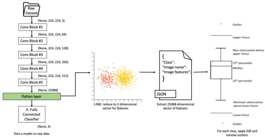
Figure 7. Pipeline for defining outlier images.
