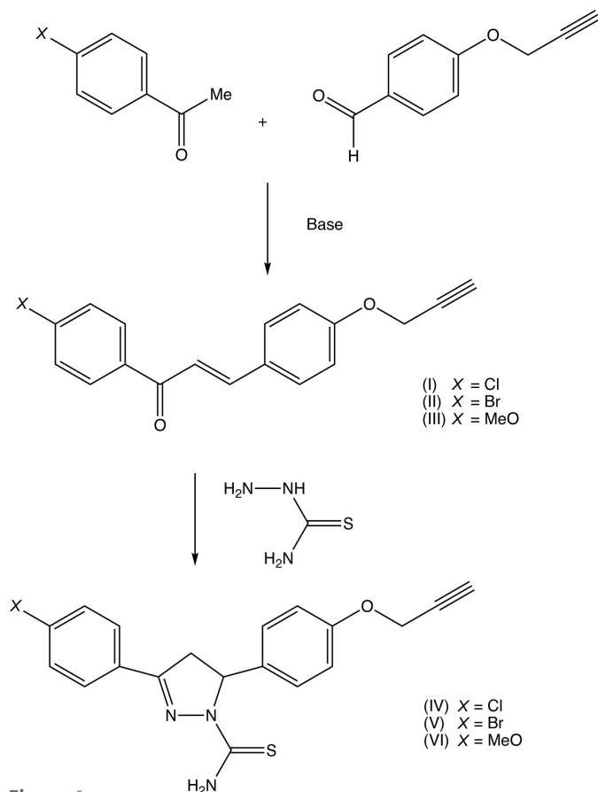
Figure 6 The synthetic route to compounds (I)–(VI).
