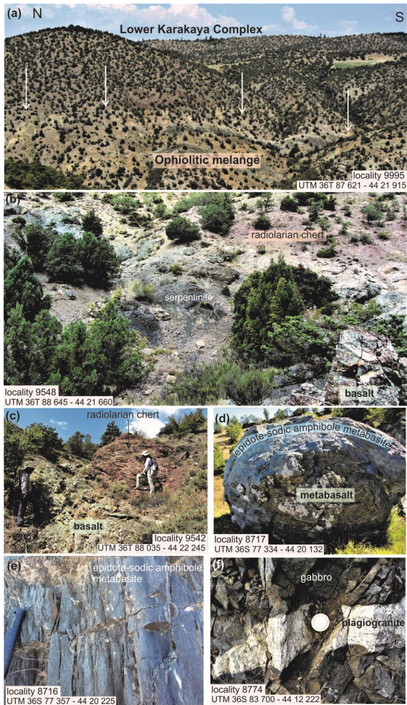
Figure 6. Photographs of the ophiolitic mélangé from the Mihaliççık region. (a) The subvertical fault contact between the Lower Karakaya Complex and the ophiolitic mélangé. (b) Red radiolarian chert, serpentinite and basalt. (c) Red radiolarian chert and basalt, the two most common rock types in the ophiolitic mélangé. (d) An incipiently metamorphosed basalt is rimmed by foliated blueschist metabasite. (e) Foliated blueschist metabasites. (f) Jurassic plagiogranite vein in gabbro. For location of the photographs see Fig. 7.
