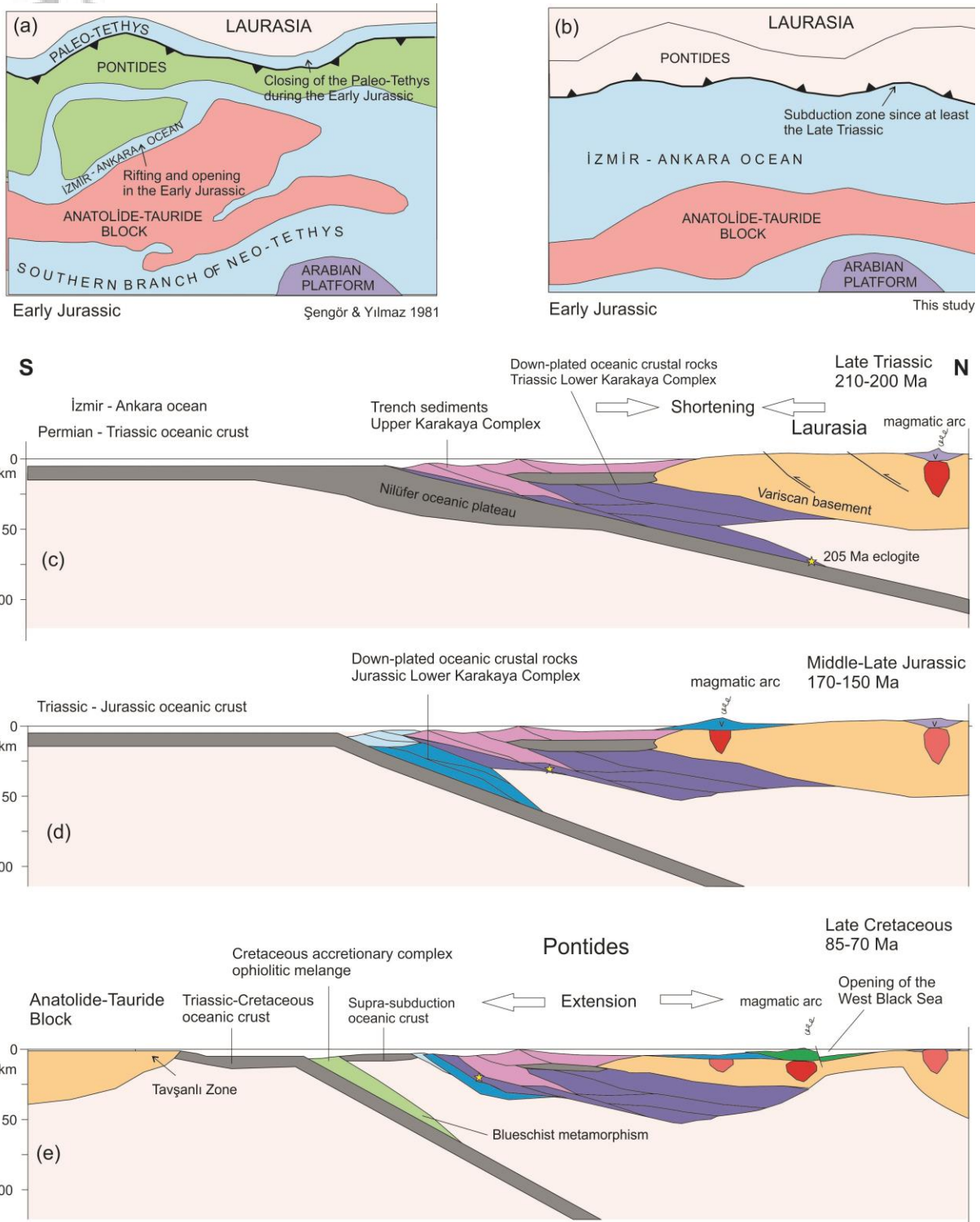
Fig. 10. (a) and (b) Sketch maps showing respective locations of the Tethyan oceans and continental units in the Early Jurassic according to Şengör & Yılmaz (1981) and the present study, respectively. (c) Collision and accretion of the Nilüfer oceanic plateau to the southern margin of Laurasia. (d) Continuing subduction and accretion during the Jurassic; in the Early Cretaceous, subduction-erosion removed most of the Jurassic subduction-accretion complex. (e) Late Cretaceous subduction-accretion. The subduction was extensional, and led to the opening of the West Black Sea basin as a back-arc. The eventual closure of the İzmir-Ankara ocean resulted in to the subduction of the continental margin of the Anatolide-Tauride Block.
