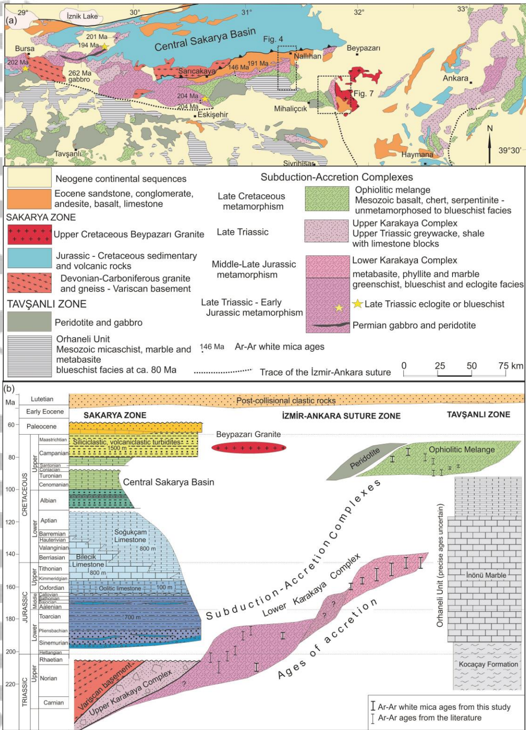
Figure 2. (a) Geological map of the İzmir-Ankara suture between Balıkesir and Ankara (based on Aksay et al., 2002; Konak, 2002; Turhan, 2002; Türkecan & Yurtsever, 2002). b. Stratigraphy of the tectonic units at the İzmir-Ankara suture zone.
