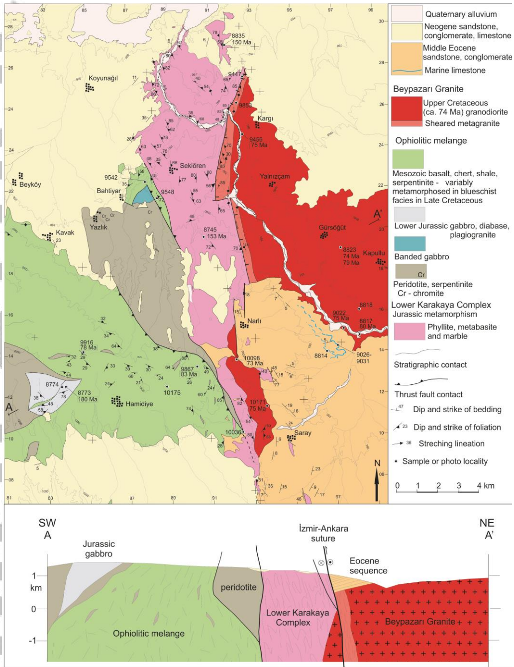
Fig. 7. Geological map and cross-section of the Mihaliçcik region. For location see Figures 1 and 2.
