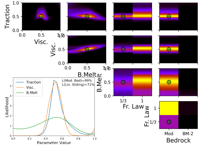
Figure 4. Likelihood of parameter combinations of synthetic test case (evaluations of Eq. (12)). Upper right panels show likelihood values marginalized to pairs of parameters, normalized to the respective maximum for clarity. Lower left panel shows likelihood values marginalized to individual parameters for the three scalar parameters (line plots), and friction law and bedrock topography map (text and quotation within), normalized to an integral of one, consistent with Probability Density Functions. The central values for traction, viscosity and ocean melt as well as nonlinear friction and modified bedrock are used. The parameter values are also shown by the black circles, while the values of the set of parameters with highest likelihood are shown by green crosses.
