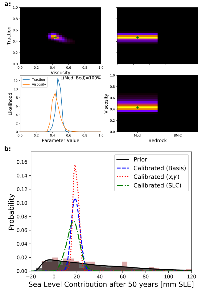
Figure 6. a: Likelihood of parameter combinations in basis representation from satellite observations (evaluations of Eq. (12)). Upper right panels show likelihood values marginalized to pairs of parameters, normalized to the respective maximum for clarity. Lower left panel shows likelihood values marginalized to individual parameters for the two scalar parameters (line plots) and bedrock topography map (text and quotation within), normalized to an integral of one in the style of Probability Density Functions. Values of the set of parameters with highest likelihood are shown by green crosses. b: Projected sea level rise contributions at the end of model period for uncalibrated BISICLES runs (brown shades), uncalibrated emulator calls (Grey shade) and different calibration approaches (colored lines).
