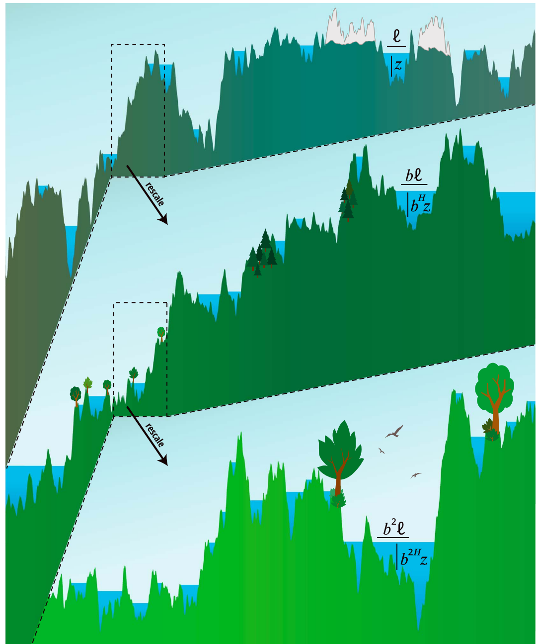
Figure 1. Schematic of statistical topographic scaling giving rise to lake volume-area scaling. Pictured is a section of a self-affine landscape with H = 0.4 . As one rescales, or “zooms in” by a factor of b horizontally and b^H vertically, the landscape is statistically identical. If lakes are passively embedded on this landscape, then lake mean depth should scale with lake area according to v \sim a^{1.2 \pm 0.05} .
