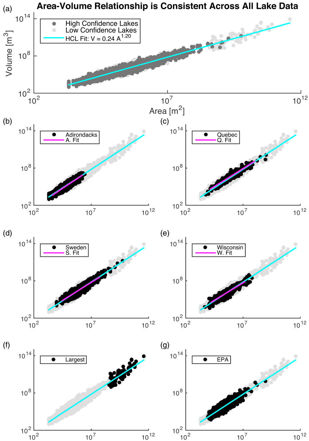
Figure 2. Volume-area scaling is consistent with Earth’s Hurst exponent across all lake data and within high-confidence lake data sets. (a) Cyan line is the OLS linear regression model of \log_{10}(\text{volume}) on \log_{10}(\text{area}) for high-confidence lakes, with a scaling estimate of 1.204, corresponding to a Hurst exponent of H = 0.41 . High-confidence lakes are plotted in dark grey, and low-confidence lakes are plotted in light grey. (b–e) Each subplot shows one high-confidence lake data set plotted in black and corresponding OLS linear regression model in magenta; compare each to cyan line. (f and g) Black points are low-confidence data sets. Residuals of high-confidence regression model prediction of low-confidence data sets are normally distributed with mean indistinguishable from zero. See supporting information. GIF of this figure is available at http://cael.space .
