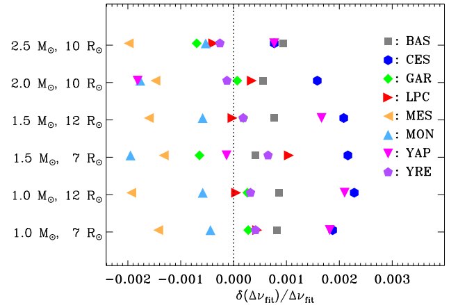
Fig. 4. Relative differences for solar-calibrated models in the large frequency separations \Delta\nu_{\text{fit}} obtained from fits to the radial-mode frequencies as functions of mode order (cf. Appendix A.3), compared with the ASTEC results, in the sense (model) – (ASTEC); the different codes are identified by the symbol shape and colour (cf. caption to Fig. 3).
