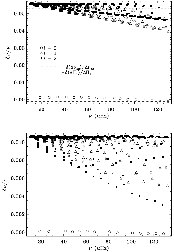
Fig. F.1. Relative differences in computed frequencies for the LPCODE 2.5 M_{\odot} , 10 R_{\odot} solar-calibrated model, compared with the ASTEC results, n' the sense (LPCODE) – (ASTEC). Top panel: original LPCODE model, bottom panel: revised model.
