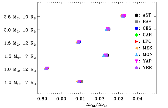
Fig. C.2. Ratios \Delta\nu_{\text{fit}}/\Delta\nu_{\text{as}} between the large frequency spacing resulting from fit to the radial-mode frequencies and the asymptotic values. The symbols correspond to the different modelling codes, as defined in the caption to Fig. 3, with the addition of AST (ASTEC). Upper panel: results for the solar-calibrated models, and lower panel: for the RGB-calibrated models.
