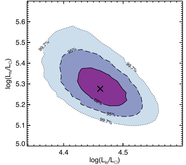
Figure 7. Probability density as a function of L_{lo} and L_{hi} when the power-law slope is constrained to \Gamma_L = -1.675 , which is the expected value for this parameter when assuming a Salpeter IMF and an MLR of L_{fin} \propto M_{init}^2 .
