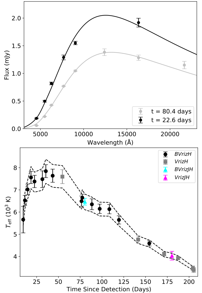
Fig. 2. Top: Two example SEDs and the best-fit reddened blackbody function. The K_s photometry is shown for the t = 80.4 d epoch, although is not included in the fitting. Bottom: Temperature evolution of AT 2019abn, as derived from SED fitting of the optical-NIR photometry and assuming E_{B-V} = 0.85 . B -band was used in the fitting when available. All BVr'i'z'H epochs shown in the plot were also fitted using Vr'i'z'H , which agreed well. For clarity we therefore only show the Vr'i'z'H fits at epochs with no B -band. The filters included in the fitting of each point are shown in the legend. The dashed lines illustrate the evolution for E_{B-V} = 0.90 (upper) and E_{B-V} = 0.79 (lower).
