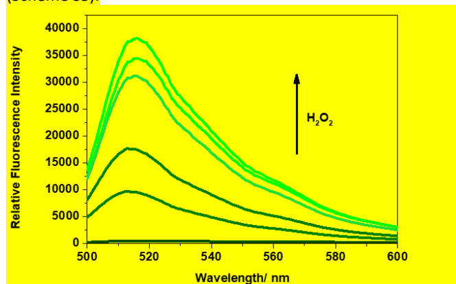
Figure 2 – Fluorescence spectra of the supernatant of Gment -based PVA-hydrogels exposed to various concentrations of \text{H}_2\text{O}_2 (0 – 1 mM) in PBS, pH 7.4. Measurements were taken after 5 min at 25 ^\circ\text{C} . \lambda_{\text{exc}} = 472 (bandwidth: 16 nm) on a BMG Labtech CLARIOstar ® plate reader.
