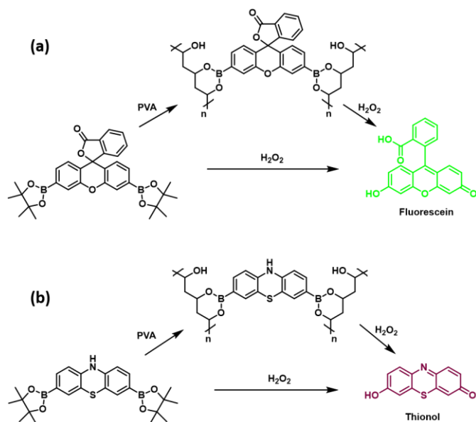
Figure 1 - (a) \text{H}_2\text{O}_2 -responsive fluorescent probe PF1 and its corresponding \text{H}_2\text{O}_2 -responsive PVA hydrogel Gment . (b) \text{H}_2\text{O}_2 -responsive fluorescent probe PT1 and its corresponding \text{H}_2\text{O}_2 -responsive PVA hydrogel Pment .
