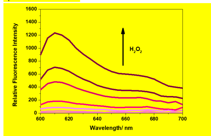
Figure 3 – Fluorescence spectra of the supernatant of Pment -based PVA-hydrogels exposed to various concentrations of \text{H}_2\text{O}_2 (0 – 1 mM) in PBS, pH 7.4. Measurements were taken after 5 min at 25 °C. \lambda_{\text{ex}} = 570 (bandwidth: 16 nm) on a BMG Labtech CLARIOstar® plate reader.
