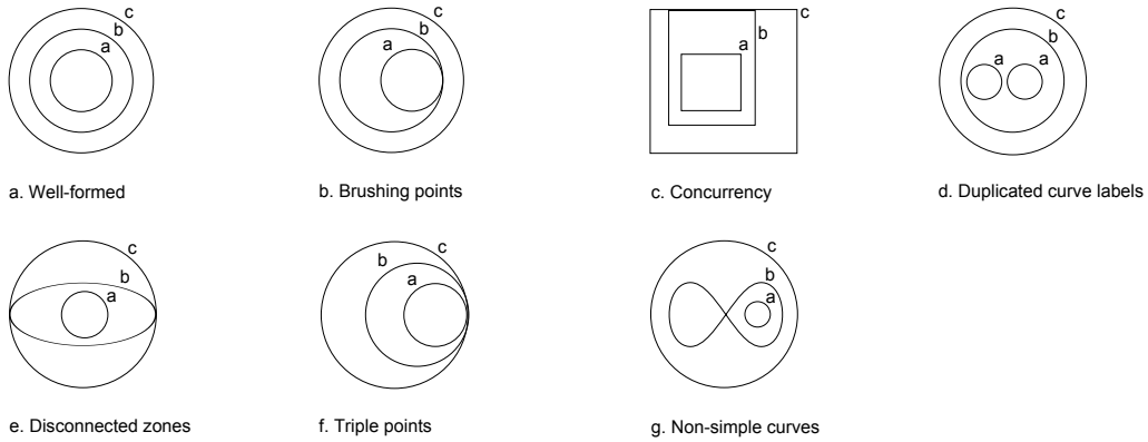
Figure 3: Non well-formed Euler diagrams.
