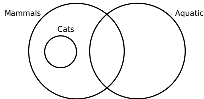
Figure 1: Simple Euler diagram.
