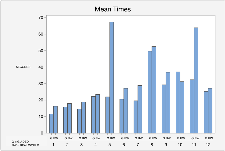
Figure 17: Comparative mean times.
