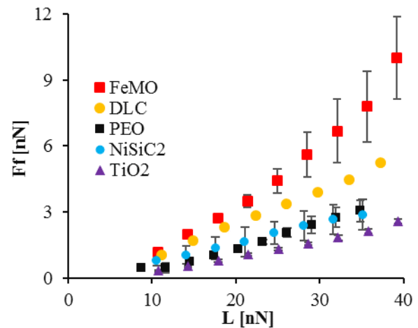
Figure 1: Friction force, F_f , vs Load, L
