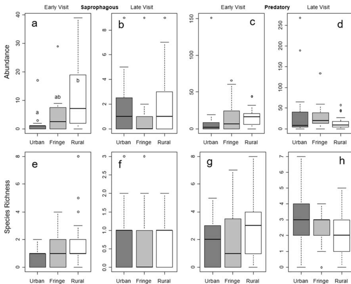
Fig. 2 Median (black bars) and inter-quartile range (shaded boxes) of (a) the abundance of saprophagous beetles during the first sampling visit, (b) abundance or saprophagous beetles during the second sampling visit, (c) abundance of predatory beetles during the first visit, (d) abundance of predatory beetles during the second visit, (e) species richness of saprophagous beetles during the first visit, (f) richness of saprophagous beetles
