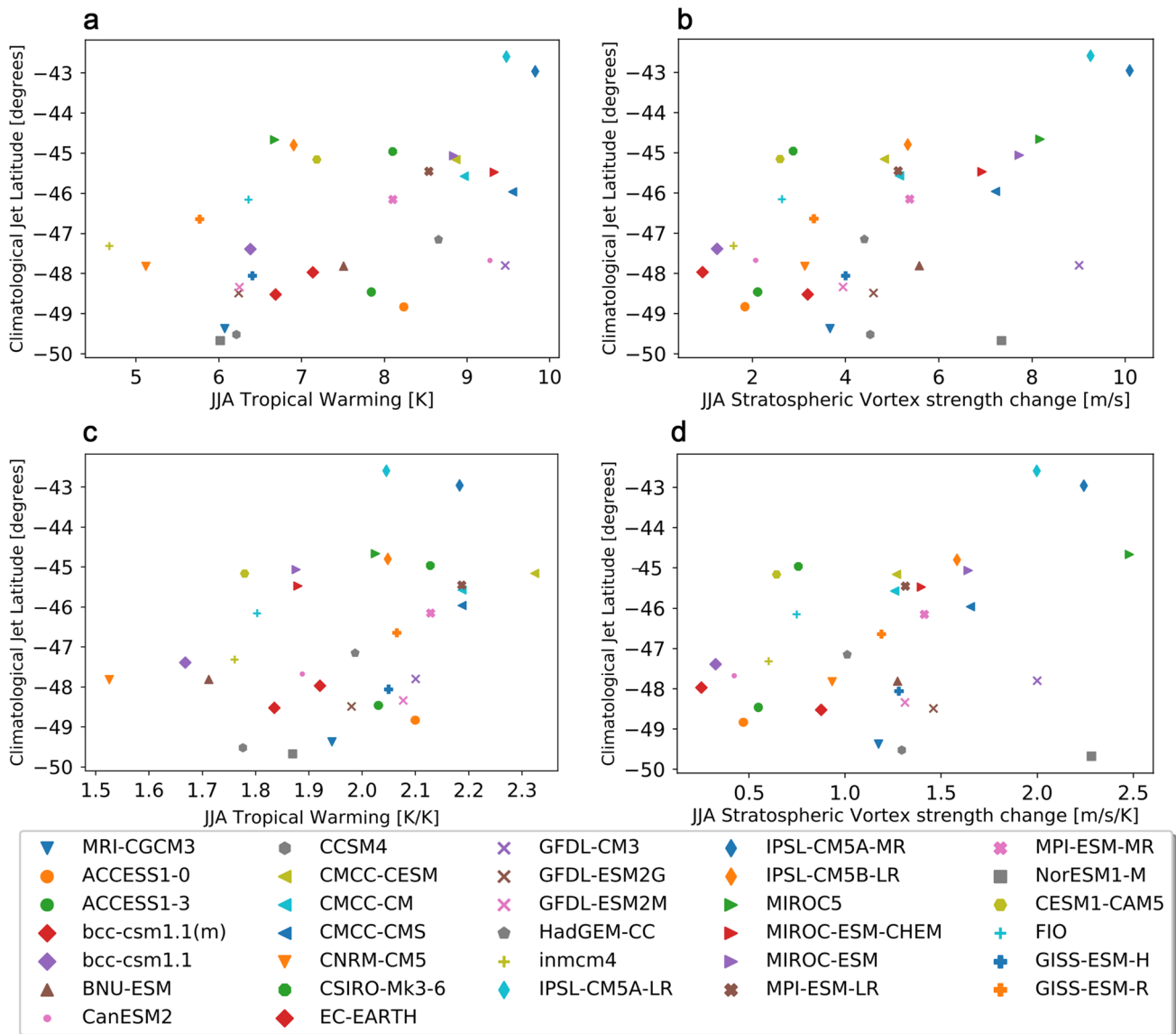
Fig. 10 Climatological position of the midlatitude jet in the historical reference period 1940–1970 vs a tropical warming, b stratospheric vortex strengthening. c, d Are the same as (a–b) but the driver indi-
