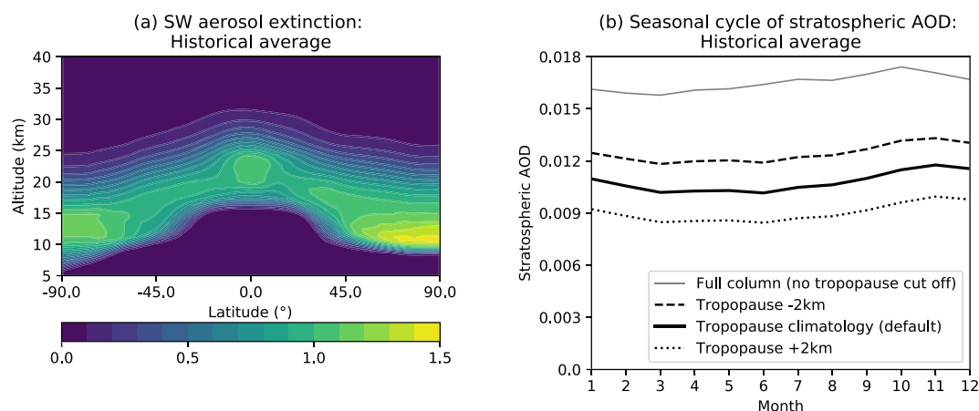
Figure 1. (a) Shortwave aerosol extinction as a function of altitude and latitude based on the annual mean from the historical average (averaged climatology used in the preindustrial control simulation and for future scenarios from 2025 onward), (b) stratospheric aerosol optical depth for the averaged climatology as function of month and depending on the implementation of tropopause height in the offline processing. Both plots show averages across the wavelength interval 0.32–0.69 \mu\text{m} .
