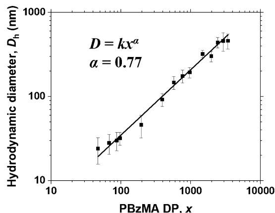
Figure 3. Hydrodynamic diameter ( D h ) vs PBzMA DP ( x ) for a series of PSMA 54 –PBzMA x diblock copolymer spheres ( x = 50–3500) prepared via RAFT dispersion polymerization of BzMA in mineral oil at 90 °C and 20% w/w. Error bars represent the standard deviation in D h as calculated from the DLS polydispersity index.
